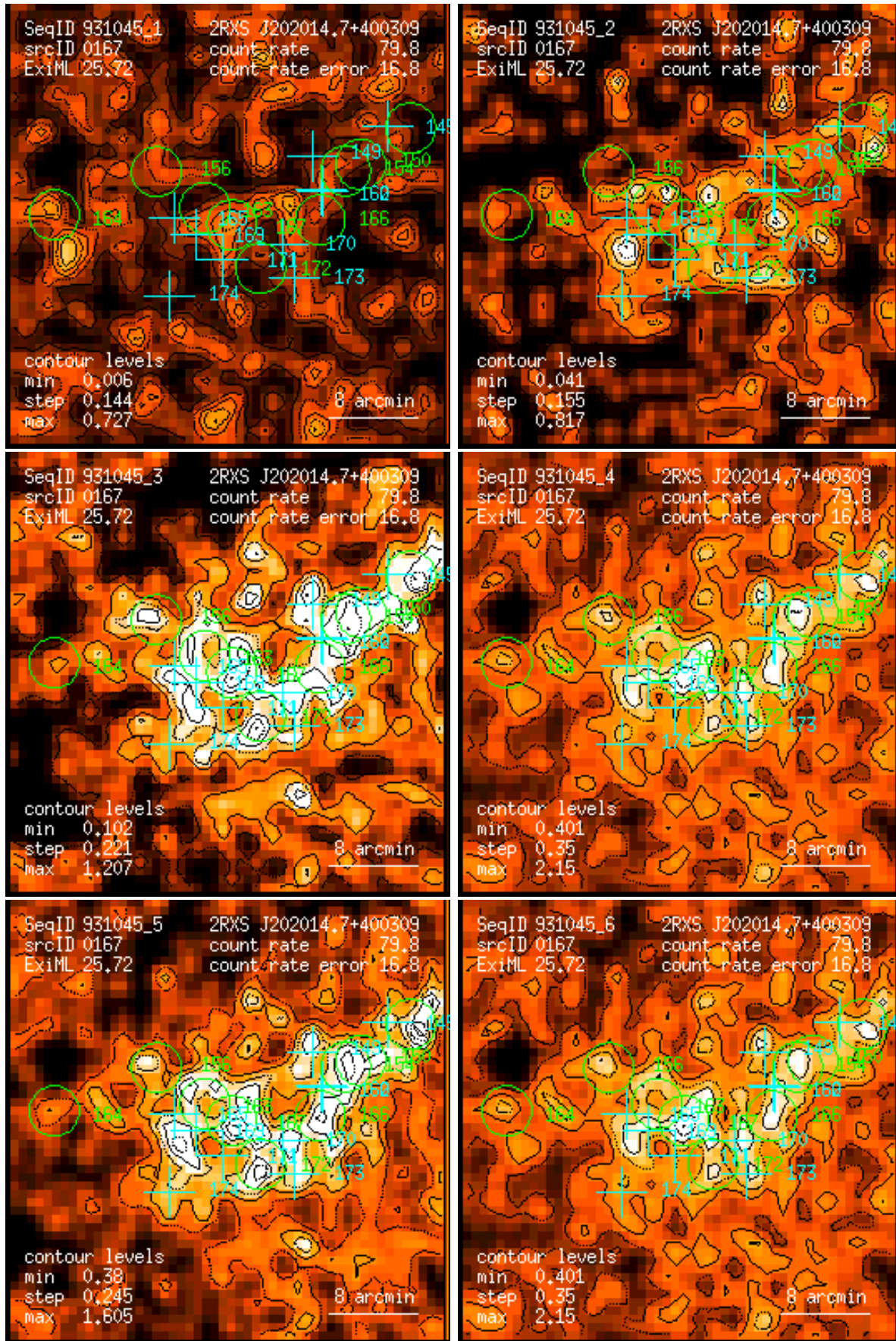
Figure 167: RASS 931045: detection 0167: band rate images, Gaussian filter: (1) PSPC channels 11 – 41, (2) 52 – 90, (3) 91 – 201, (4) 11 – 235, (5) 52 – 201, (6) 11 – 201. Broad band rates in counts/ks. Band rate contour levels in counts/ks/arcmin 2 .
