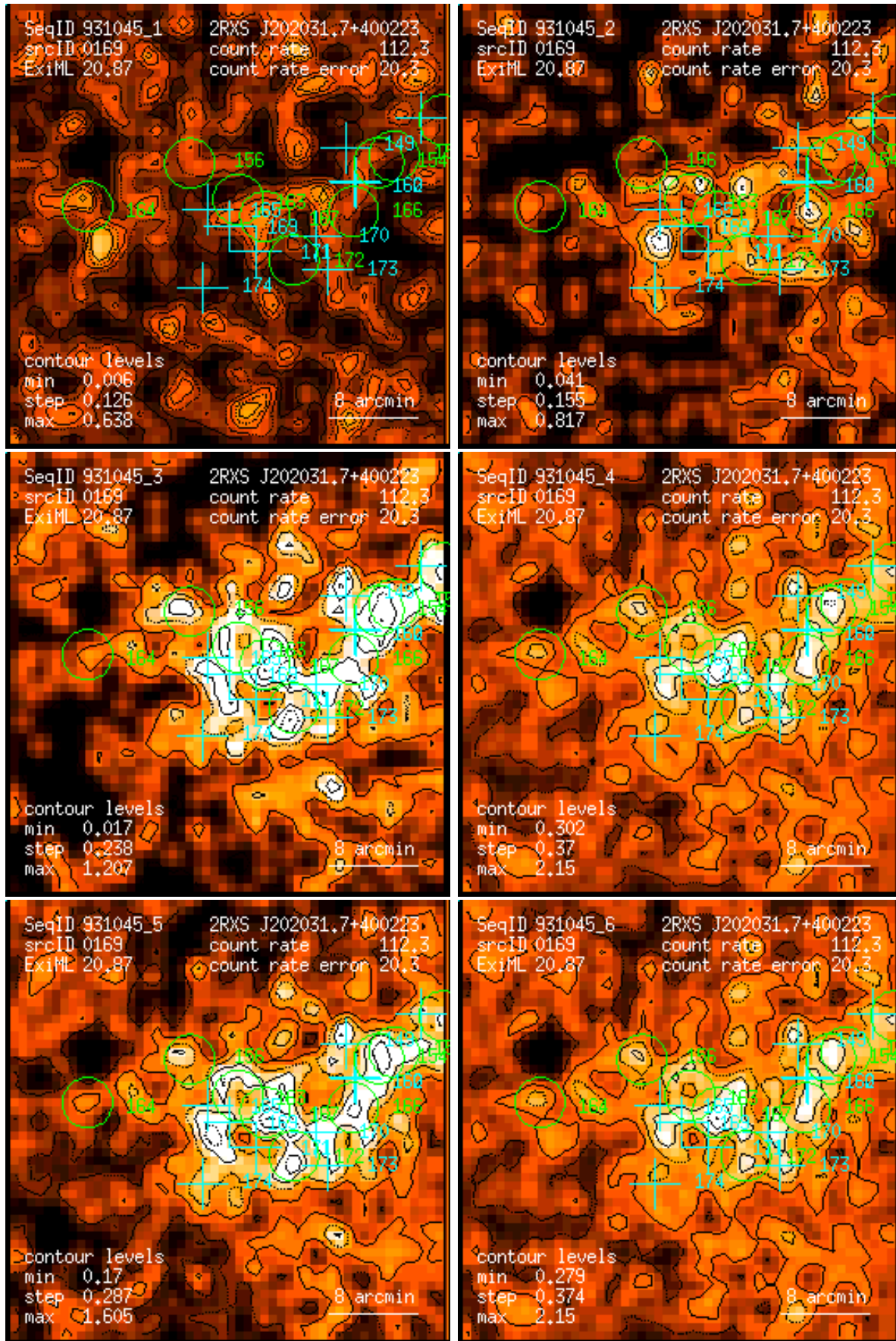
Figure 169: RASS 931045: detection 0169: band rate images, Gaussian filter: (1) PSPC channels 11 – 41, (2) 52 – 90, (3) 91 – 201, (4) 11 – 235, (5) 52 – 201, (6) 11 – 201. Broad band rates in counts/ks. Band rate contour levels in counts/ks/arcmin 2 .
