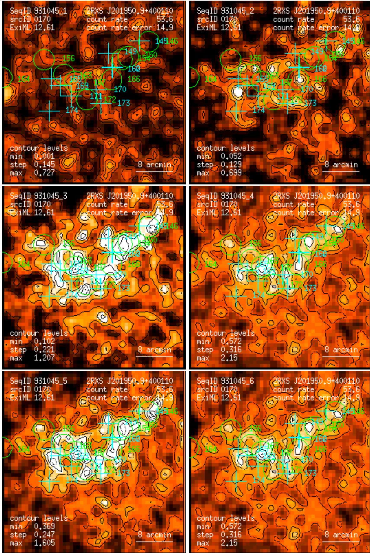
Figure 170: RASS 931045: detection 0170: band rate images, Gaussian filter: (1) PSPC channels 11 – 41, (2) 52 – 90, (3) 91 – 201, (4) 11 – 235, (5) 52 – 201, (6) 11 – 201. Broad band rates in counts/ks. Band rate contour levels in counts/ks/arcmin 2 .
