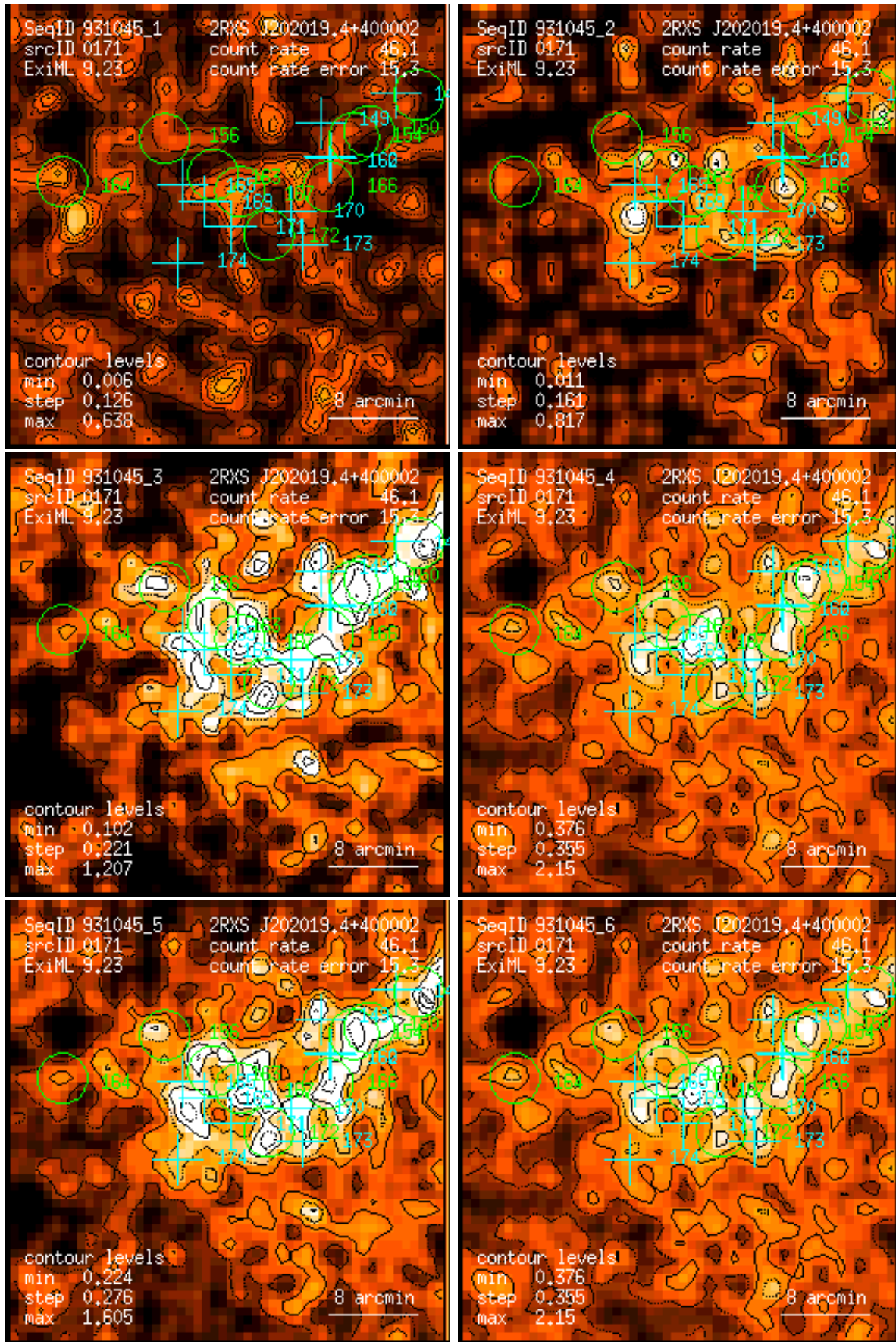
Figure 171: RASS 931045: detection 0171: band rate images, Gaussian filter: (1) PSPC channels 11 – 41, (2) 52 – 90, (3) 91 – 201, (4) 11 – 235, (5) 52 – 201, (6) 11 – 201. Broad band rates in counts/ks. Band rate contour levels in counts/ks/arcmin 2 .
