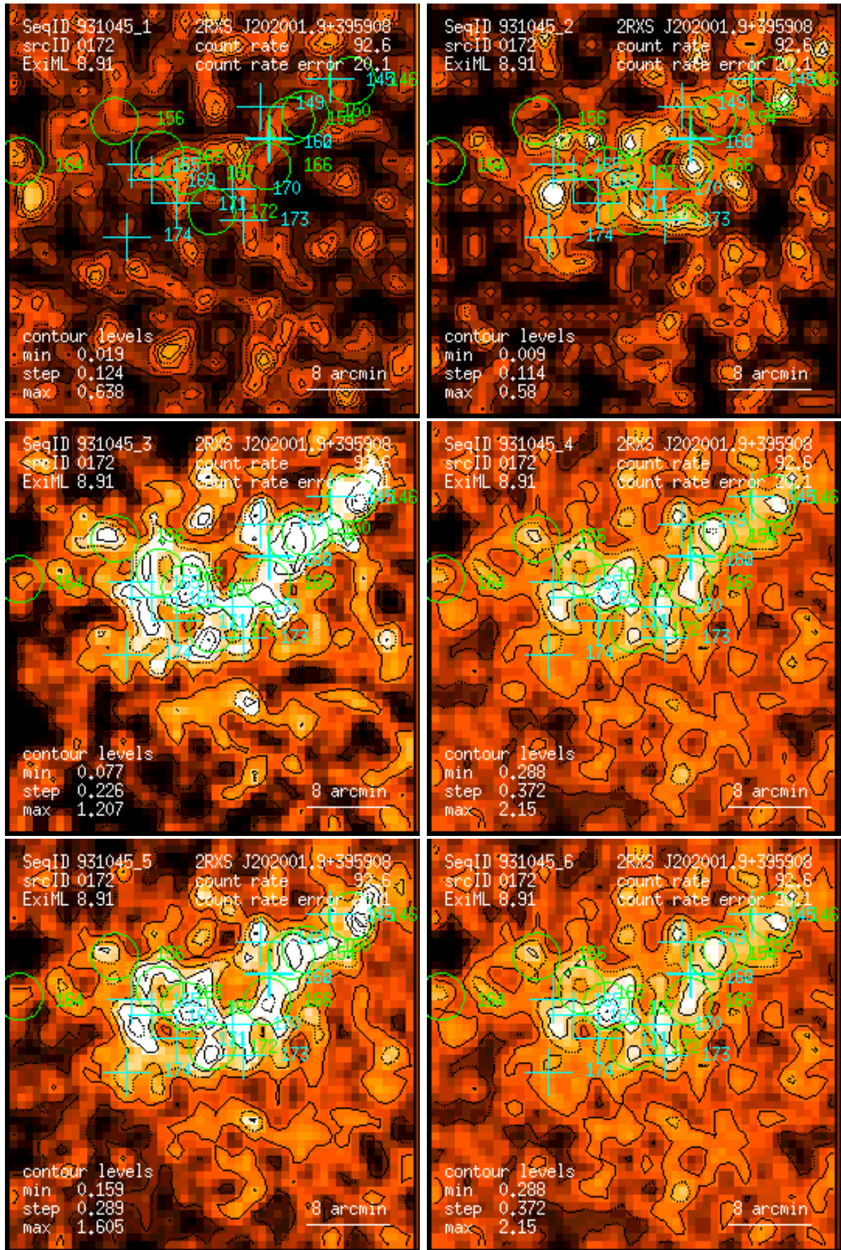
Figure 172: RASS 931045: detection 0172: band rate images, Gaussian filter: (1) PSPC channels 11 – 41, (2) 52 – 90, (3) 91 – 201, (4) 11 – 235, (5) 52 – 201, (6) 11 – 201. Broad band rates in counts/ks. Band rate contour levels in counts/ks/arcmin 2 .
