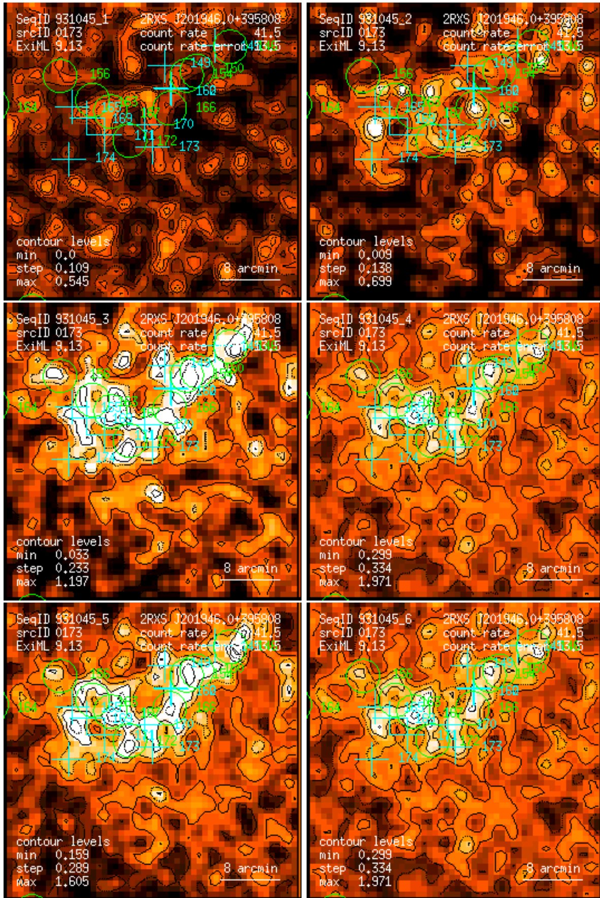
Figure 173: RASS 931045: detection 0173: band rate images, Gaussian filter: (1) PSPC channels 11 – 41, (2) 52 – 90, (3) 91 – 201, (4) 11 – 235, (5) 52 – 201, (6) 11 – 201. Broad band rates in counts/ks. Band rate contour levels in counts/ks/arcmin 2 .
