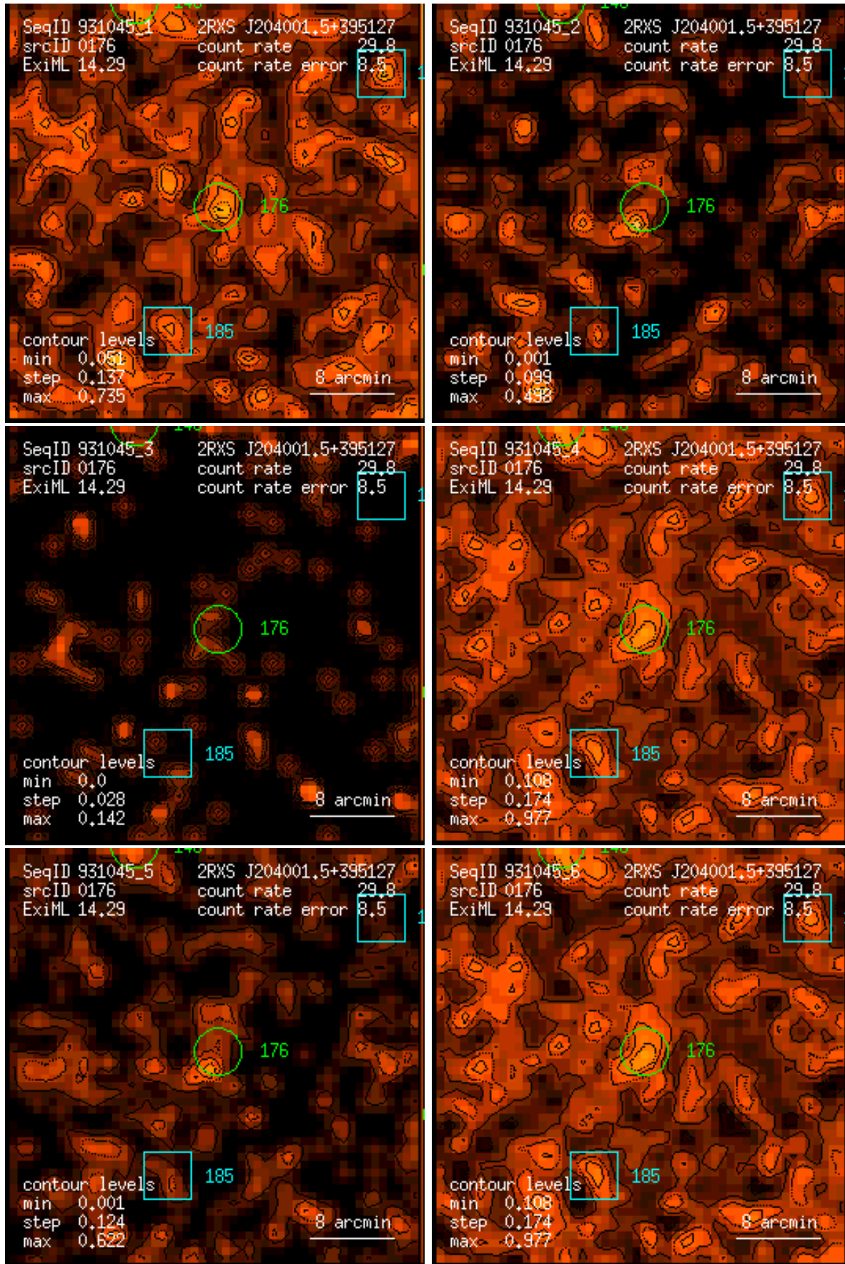
Figure 176: RASS 931045: detection 0176: band rate images, Gaussian filter: (1) PSPC channels 11 – 41, (2) 52 – 90, (3) 91 – 201, (4) 11 – 235, (5) 52 – 201, (6) 11 – 201. Broad band rates in counts/ks. Band rate contour levels in counts/ks/arcmin 2 .
