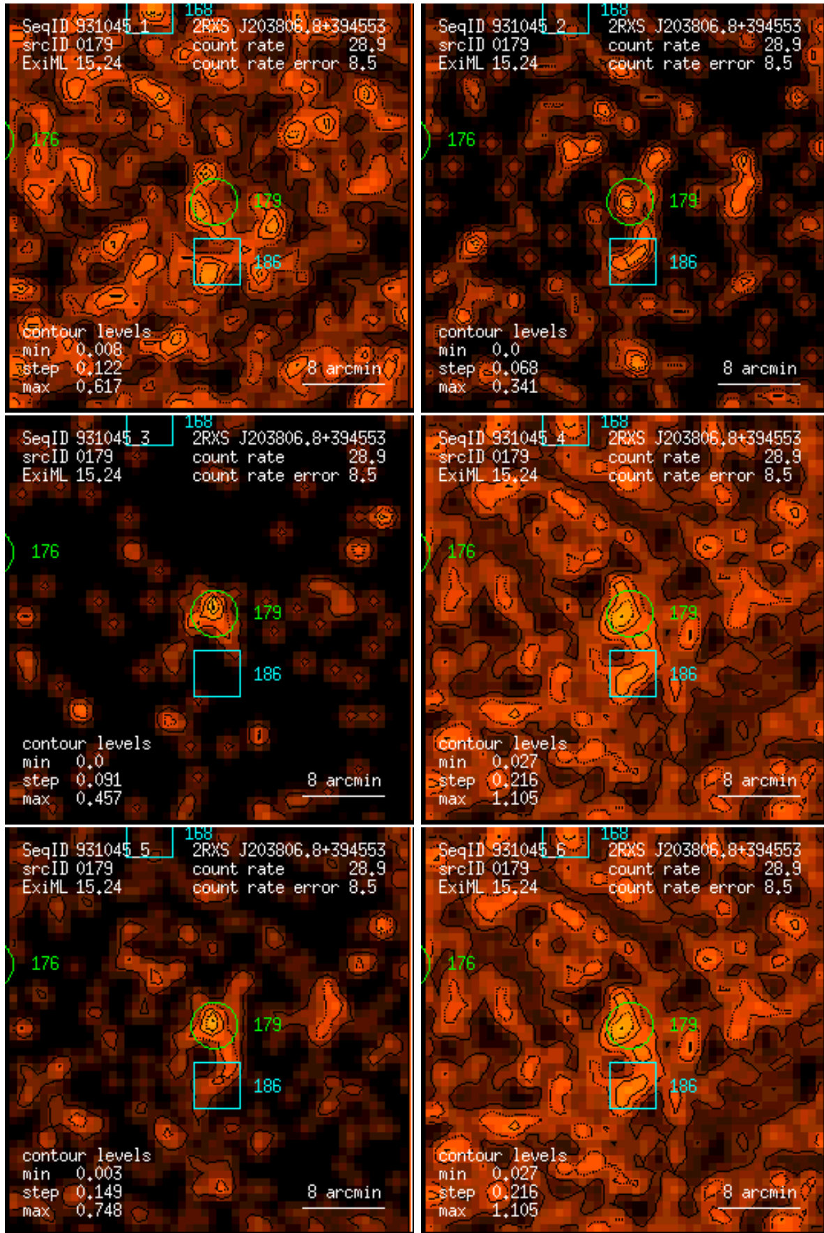
Figure 179: RASS 931045: detection 0179: band rate images, Gaussian filter: (1) PSPC channels 11 – 41, (2) 52 – 90, (3) 91 – 201, (4) 11 – 235, (5) 52 – 201, (6) 11 – 201. Broad band rates in counts/ks. Band rate contour levels in counts/ks/arcmin 2 .
