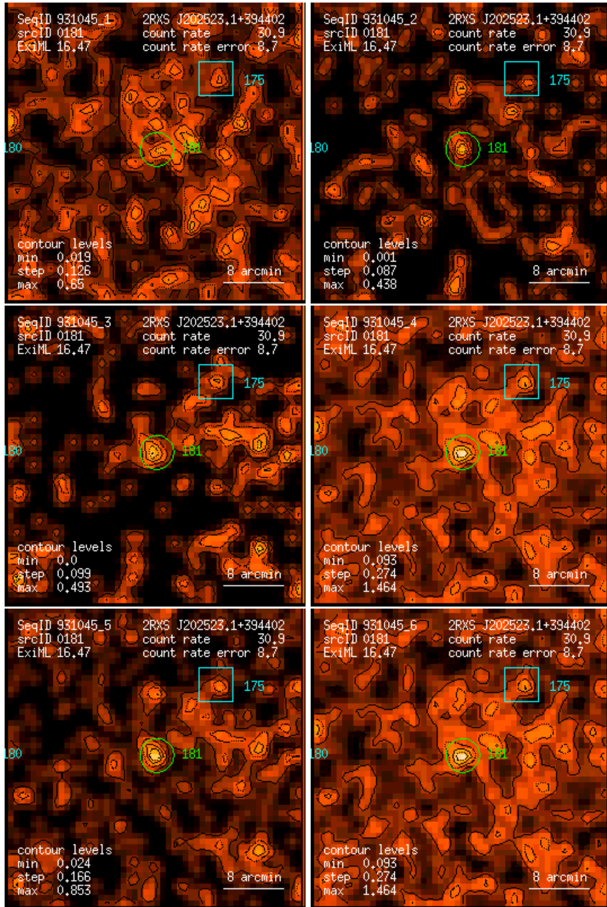
Figure 181: RASS 931045: detection 0181: band rate images, Gaussian filter: (1) PSPC channels 11 – 41, (2) 52 – 90, (3) 91 – 201, (4) 11 – 235, (5) 52 – 201, (6) 11 – 201. Broad band rates in counts/ks. Band rate contour levels in counts/ks/arcmin 2 .
