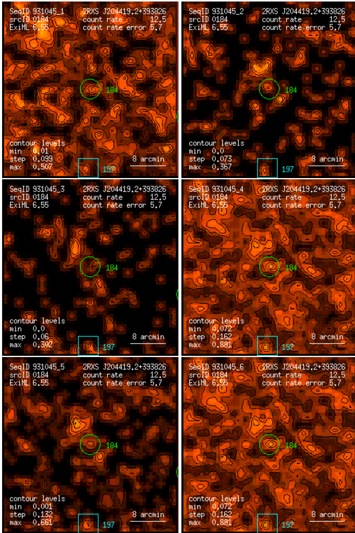
Figure 184: RASS 931045: detection 0184: band rate images, Gaussian filter: (1) PSPC channels 11 – 41, (2) 52 – 90, (3) 91 – 201, (4) 11 – 235, (5) 52 – 201, (6) 11 – 201. Broad band rates in counts/ks. Band rate contour levels in counts/ks/arcmin 2 .
