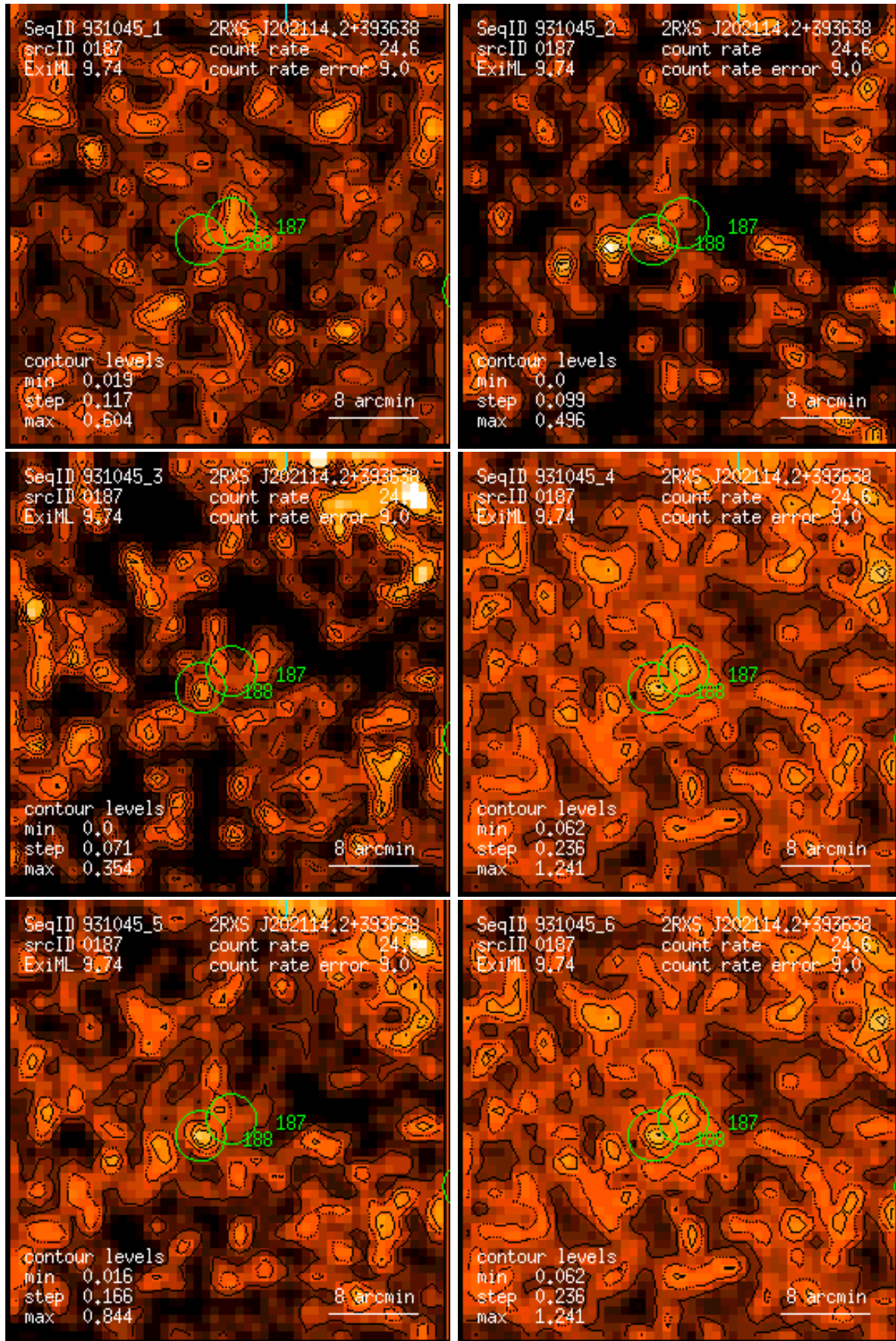
Figure 187: RASS 931045: detection 0187: band rate images, Gaussian filter: (1) PSPC channels 11 – 41, (2) 52 – 90, (3) 91 – 201, (4) 11 – 235, (5) 52 – 201, (6) 11 – 201. Broad band rates in counts/ks. Band rate contour levels in counts/ks/arcmin 2 .
