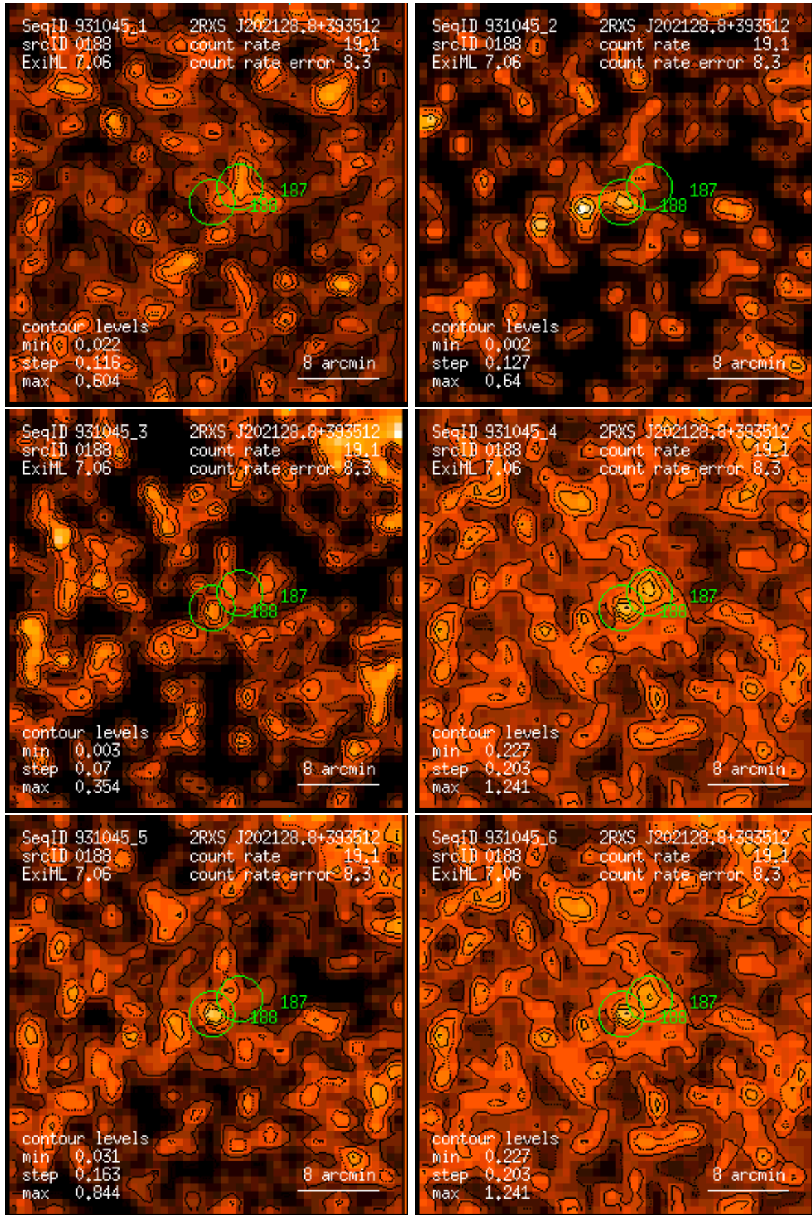
Figure 188: RASS 931045: detection 0188: band rate images, Gaussian filter: (1) PSPC channels 11 – 41, (2) 52 – 90, (3) 91 – 201, (4) 11 – 235, (5) 52 – 201, (6) 11 – 201. Broad band rates in counts/ks. Band rate contour levels in counts/ks/arcmin 2 .
