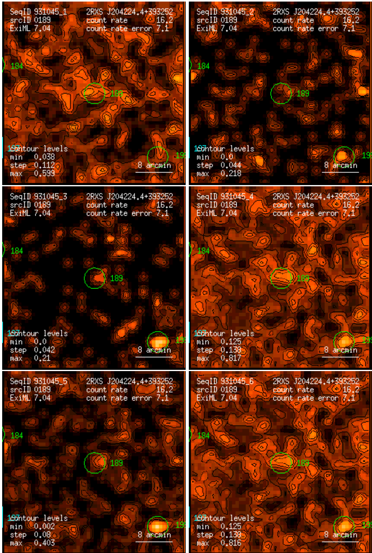
Figure 189: RASS 931045: detection 0189: band rate images, Gaussian filter: (1) PSPC channels 11 – 41, (2) 52 – 90, (3) 91 – 201, (4) 11 – 235, (5) 52 – 201, (6) 11 – 201. Broad band rates in counts/ks. Band rate contour levels in counts/ks/arcmin 2 .
