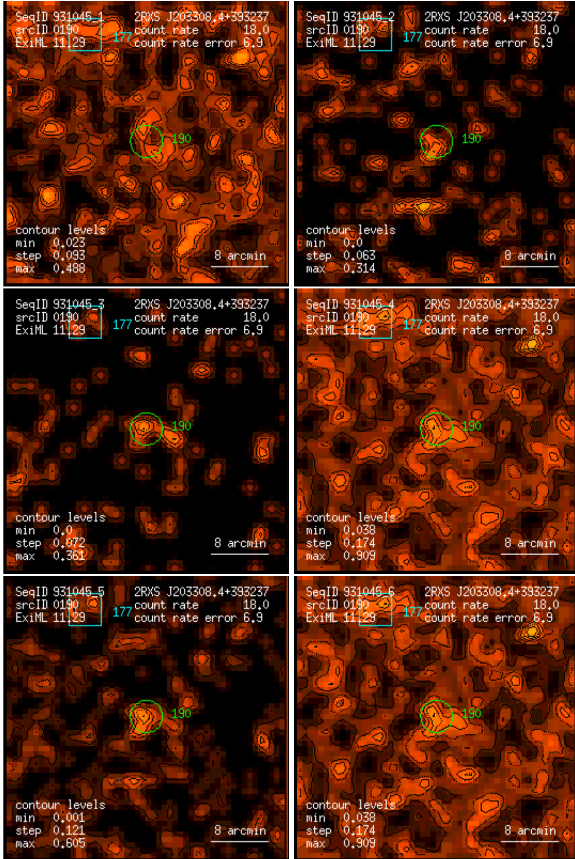
Figure 190: RASS 931045: detection 0190: band rate images, Gaussian filter: (1) PSPC channels 11 – 41, (2) 52 – 90, (3) 91 – 201, (4) 11 – 235, (5) 52 – 201, (6) 11 – 201. Broad band rates in counts/ks. Band rate contour levels in counts/ks/arcmin 2 .
