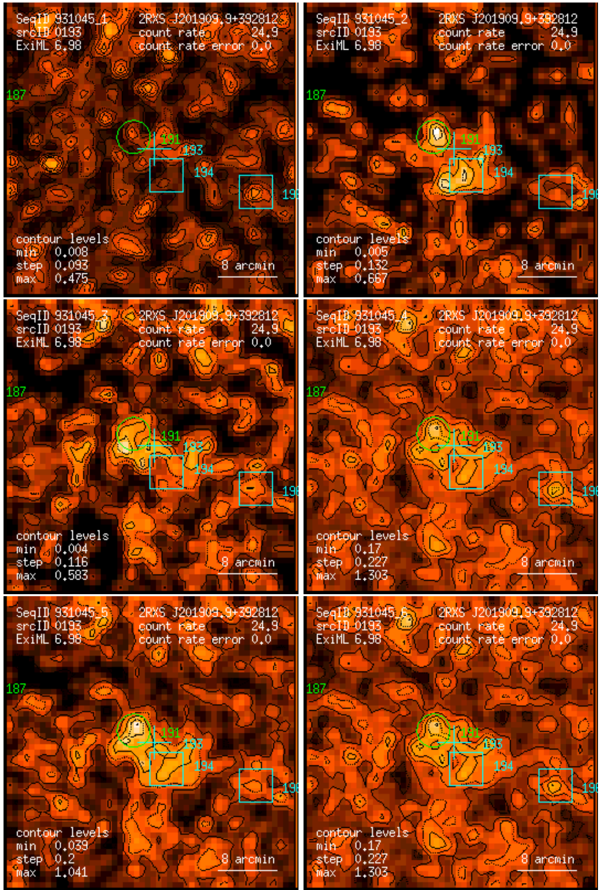
Figure 193: RASS 931045: detection 0193: band rate images, Gaussian filter: (1) PSPC channels 11 – 41, (2) 52 – 90, (3) 91 – 201, (4) 11 – 235, (5) 52 – 201, (6) 11 – 201. Broad band rates in counts/ks. Band rate contour levels in counts/ks/arcmin 2 .
