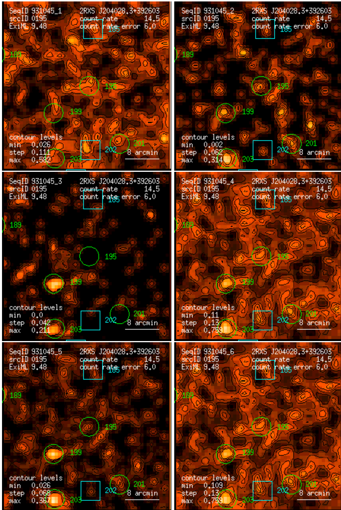
Figure 195: RASS 931045: detection 0195: band rate images, Gaussian filter: (1) PSPC channels 11 – 41, (2) 52 – 90, (3) 91 – 201, (4) 11 – 235, (5) 52 – 201, (6) 11 – 201. Broad band rates in counts/ks. Band rate contour levels in counts/ks/arcmin 2 .
