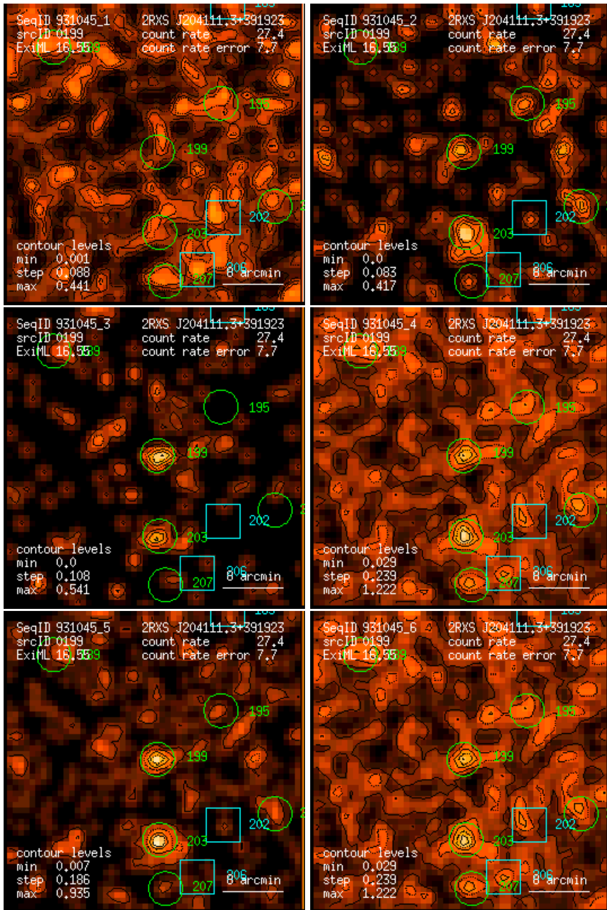
Figure 199: RASS 931045: detection 0199: band rate images, Gaussian filter: (1) PSPC channels 11 – 41, (2) 52 – 90, (3) 91 – 201, (4) 11 – 235, (5) 52 – 201, (6) 11 – 201. Broad band rates in counts/ks. Band rate contour levels in counts/ks/arcmin 2 .
