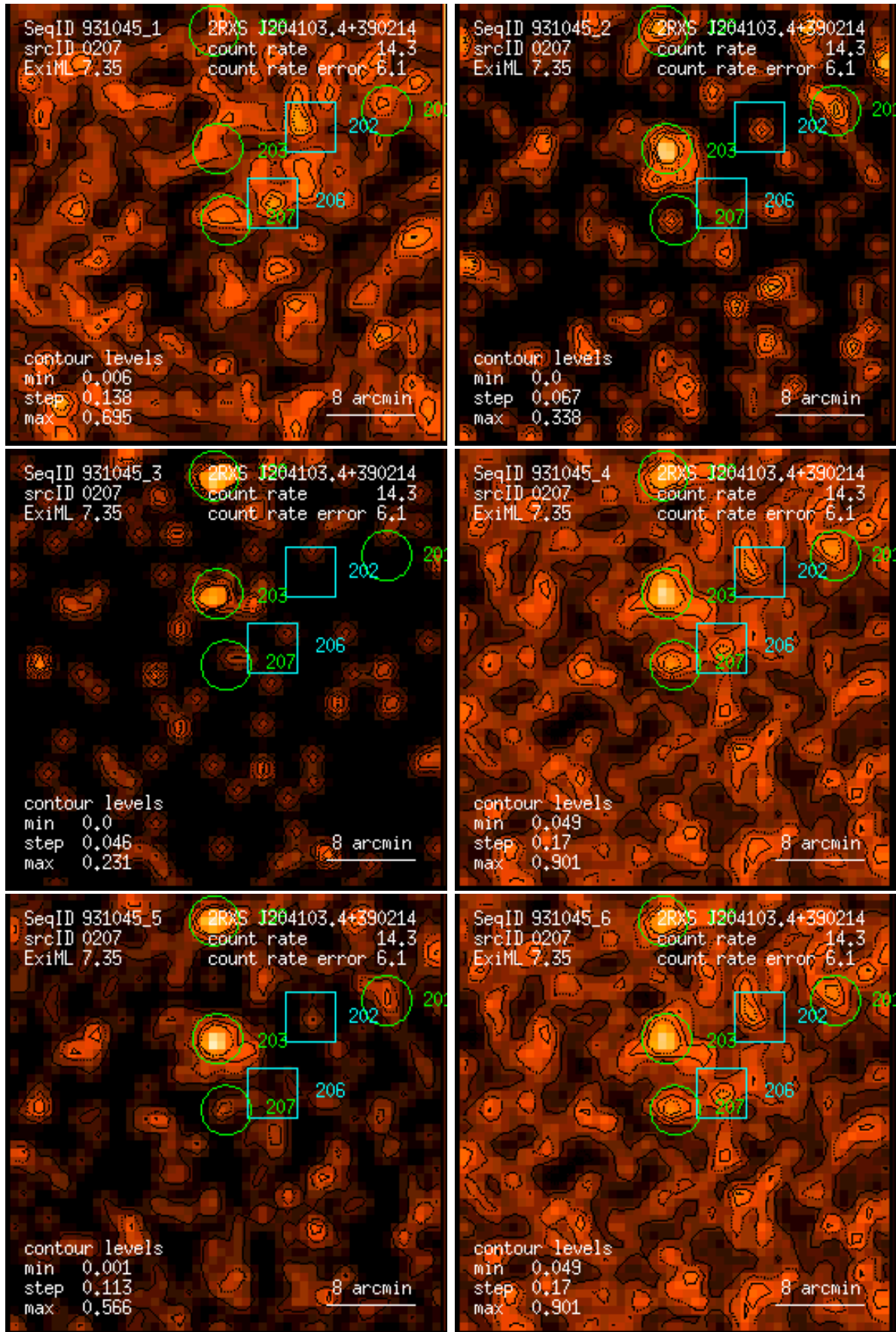
Figure 207: RASS 931045: detection 0207: band rate images, Gaussian filter: (1) PSPC channels 11 – 41, (2) 52 – 90, (3) 91 – 201, (4) 11 – 235, (5) 52 – 201, (6) 11 – 201. Broad band rates in counts/ks. Band rate contour levels in counts/ks/arcmin 2 .
