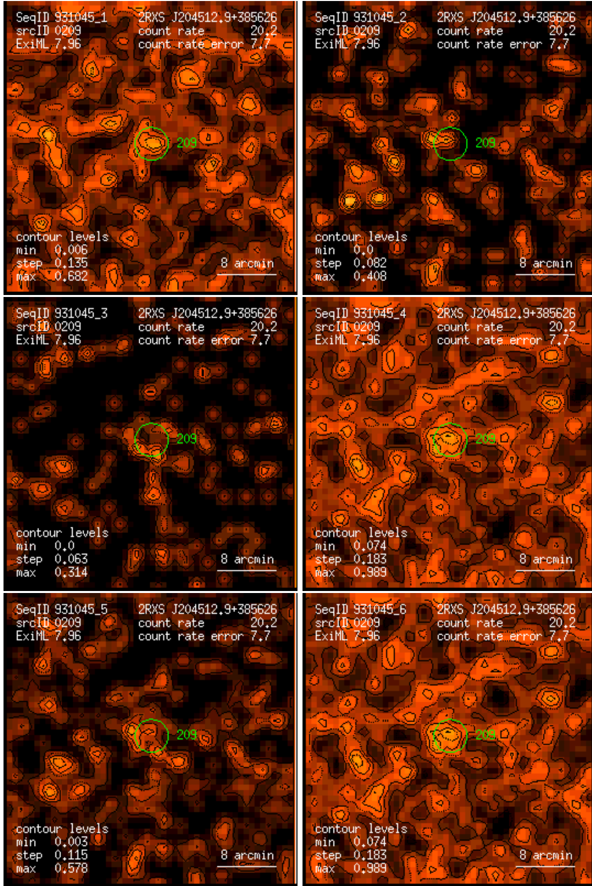
Figure 209: RASS 931045: detection 0209: band rate images, Gaussian filter: (1) PSPC channels 11 – 41, (2) 52 – 90, (3) 91 – 201, (4) 11 – 235, (5) 52 – 201, (6) 11 – 201. Broad band rates in counts/ks. Band rate contour levels in counts/ks/arcmin 2 .
