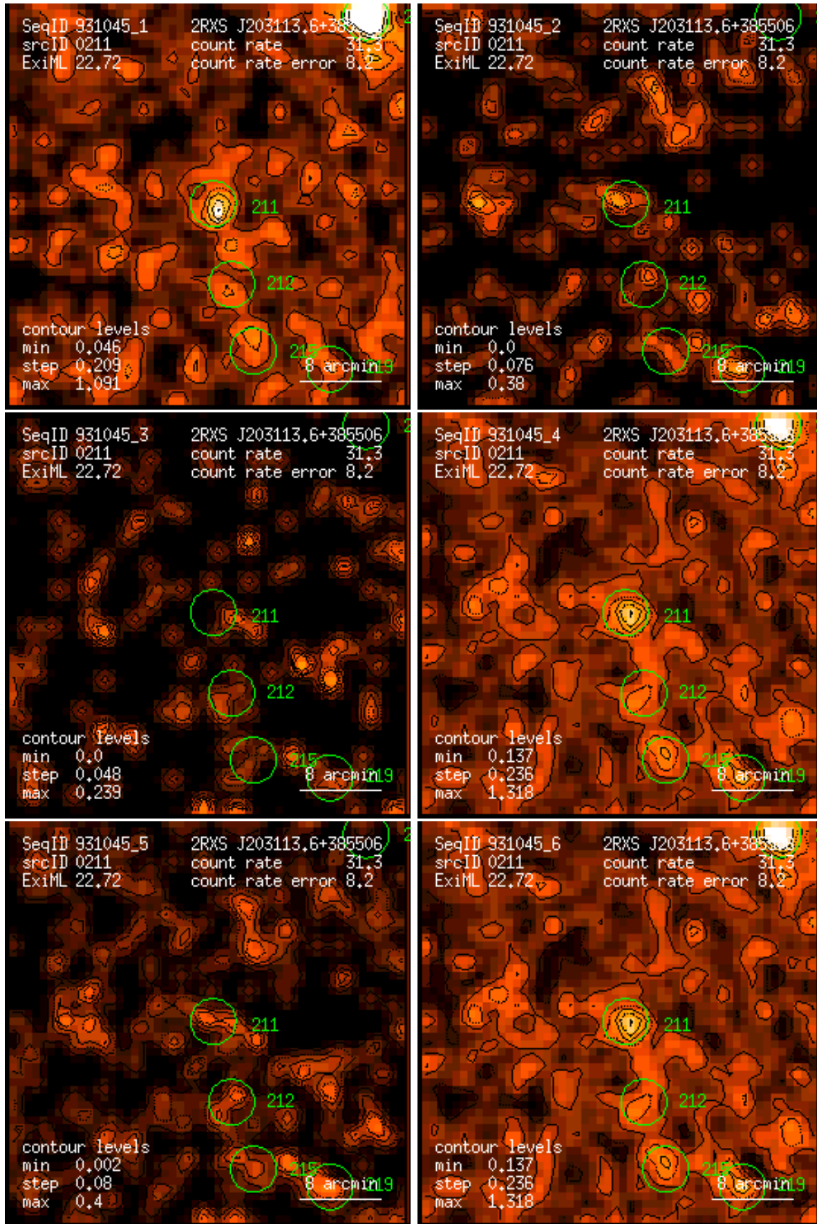
Figure 211: RASS 931045: detection 0211: band rate images, Gaussian filter: (1) PSPC channels 11 – 41, (2) 52 – 90, (3) 91 – 201, (4) 11 – 235, (5) 52 – 201, (6) 11 – 201. Broad band rates in counts/ks. Band rate contour levels in counts/ks/arcmin 2 .
