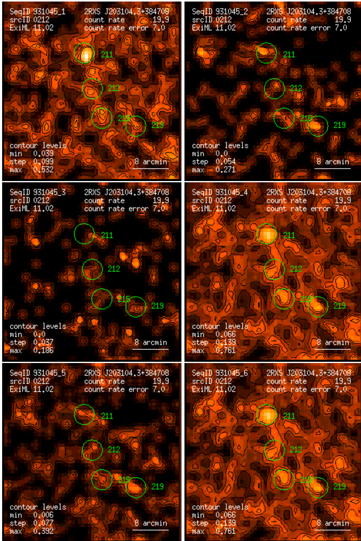
Figure 212: RASS 931045: detection 0212: band rate images, Gaussian filter: (1) PSPC channels 11 – 41, (2) 52 – 90, (3) 91 – 201, (4) 11 – 235, (5) 52 – 201, (6) 11 – 201. Broad band rates in counts/ks. Band rate contour levels in counts/ks/arcmin 2 .
