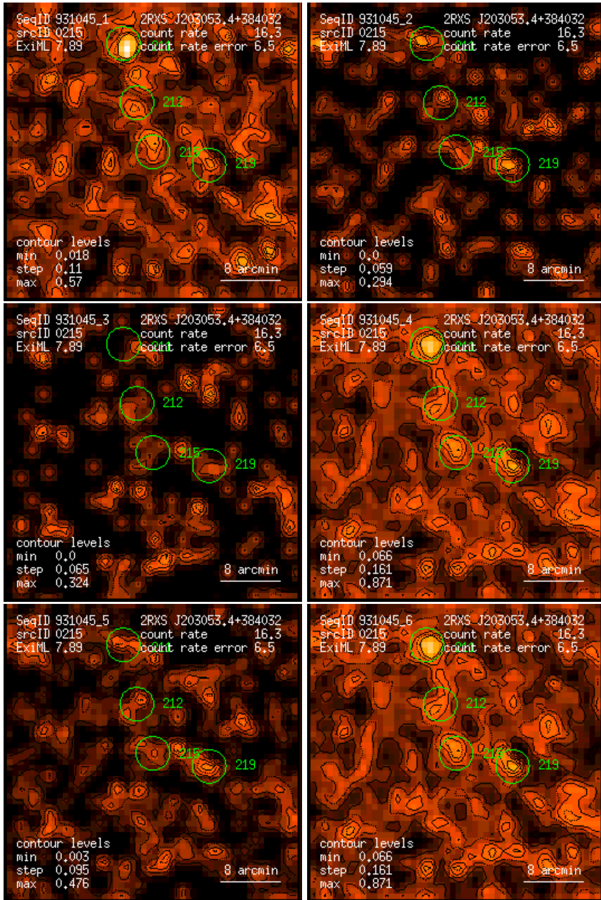
Figure 215: RASS 931045: detection 0215: band rate images, Gaussian filter: (1) PSPC channels 11 – 41, (2) 52 – 90, (3) 91 – 201, (4) 11 – 235, (5) 52 – 201, (6) 11 – 201. Broad band rates in counts/ks. Band rate contour levels in counts/ks/arcmin 2 .
