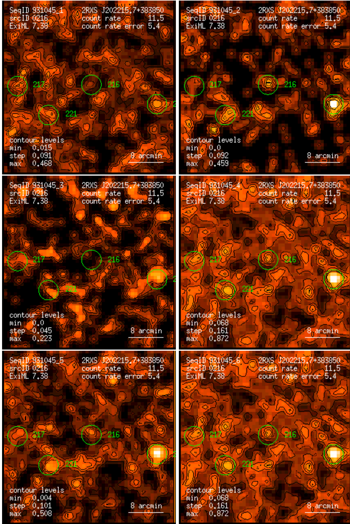
Figure 216: RASS 931045: detection 0216: band rate images, Gaussian filter: (1) PSPC channels 11 – 41, (2) 52 – 90, (3) 91 – 201, (4) 11 – 235, (5) 52 – 201, (6) 11 – 201. Broad band rates in counts/ks. Band rate contour levels in counts/ks/arcmin 2 .
