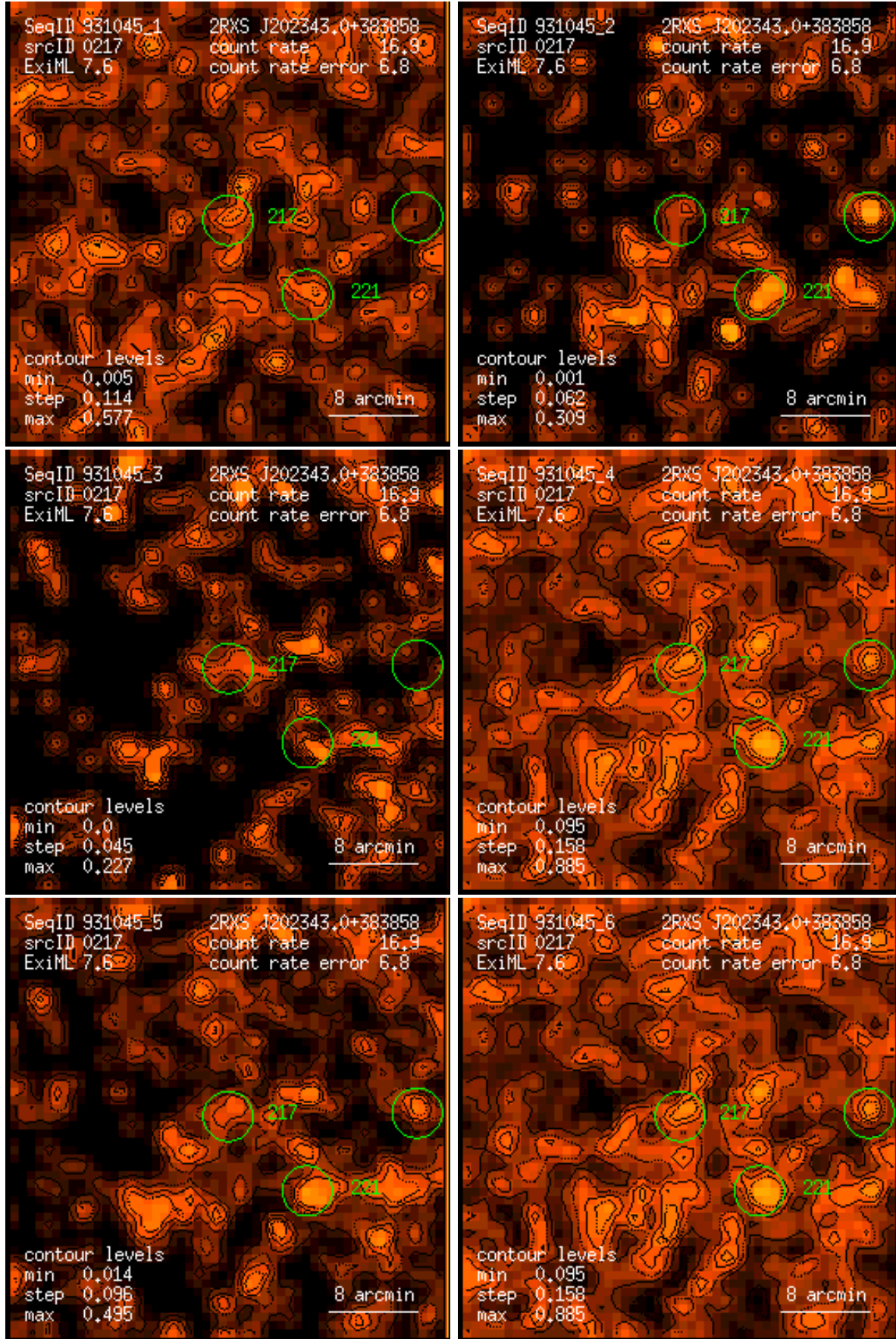
Figure 217: RASS 931045: detection 0217: band rate images, Gaussian filter: (1) PSPC channels 11 – 41, (2) 52 – 90, (3) 91 – 201, (4) 11 – 235, (5) 52 – 201, (6) 11 – 201. Broad band rates in counts/ks. Band rate contour levels in counts/ks/arcmin 2 .
