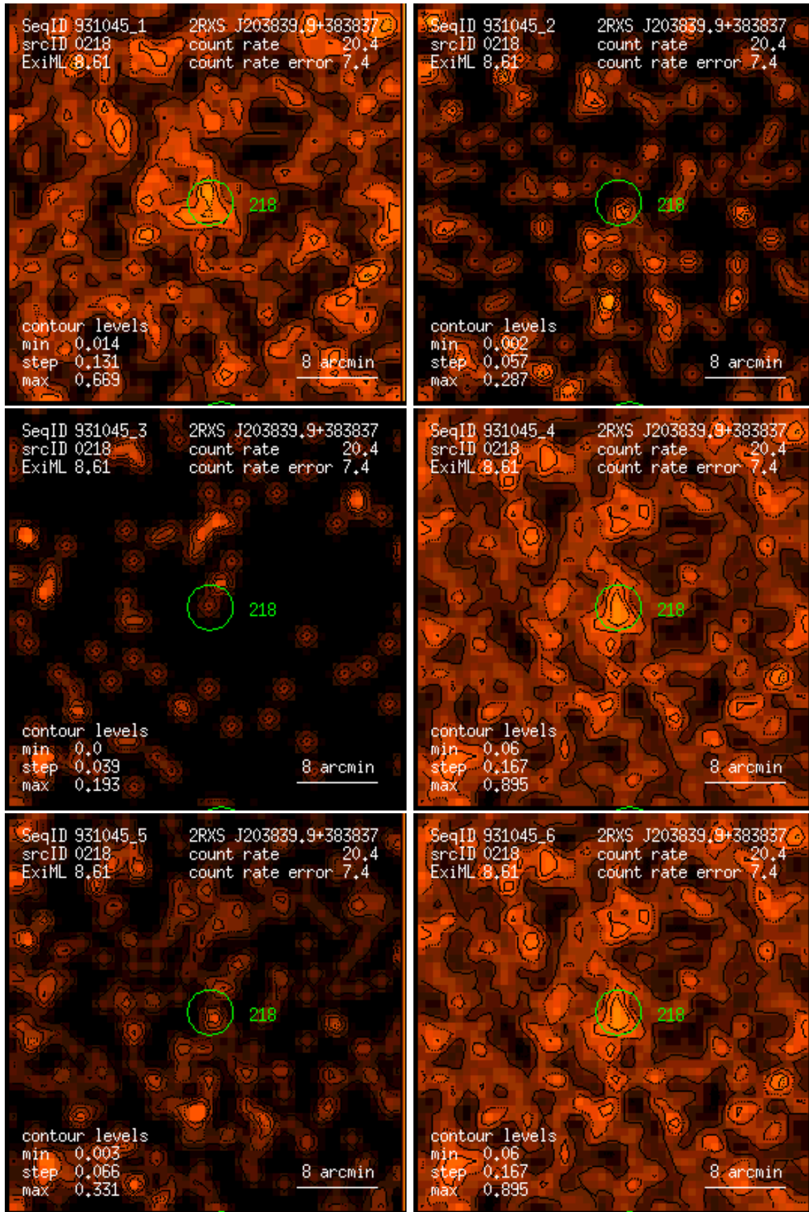
Figure 218: RASS 931045: detection 0218: band rate images, Gaussian filter: (1) PSPC channels 11 – 41, (2) 52 – 90, (3) 91 – 201, (4) 11 – 235, (5) 52 – 201, (6) 11 – 201. Broad band rates in counts/ks. Band rate contour levels in counts/ks/arcmin 2 .
