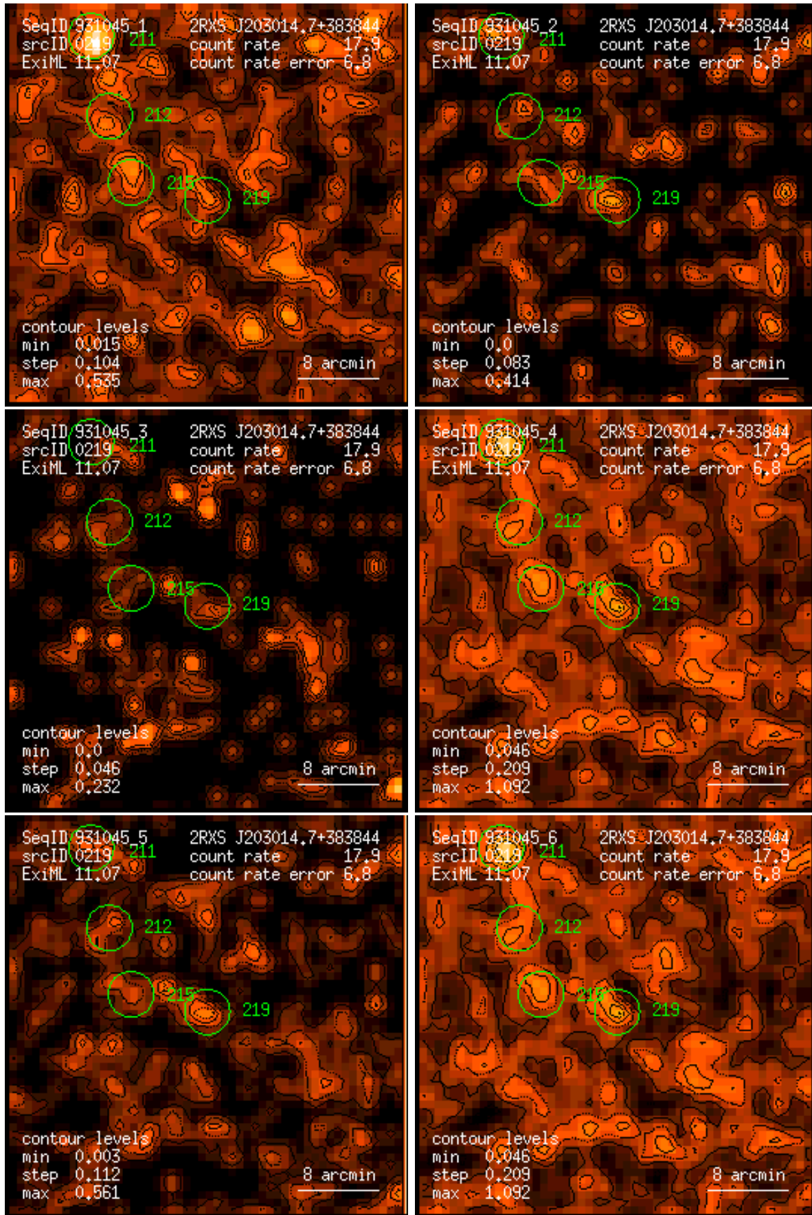
Figure 219: RASS 931045: detection 0219: band rate images, Gaussian filter: (1) PSPC channels 11 – 41, (2) 52 – 90, (3) 91 – 201, (4) 11 – 235, (5) 52 – 201, (6) 11 – 201. Broad band rates in counts/ks. Band rate contour levels in counts/ks/arcmin 2 .
