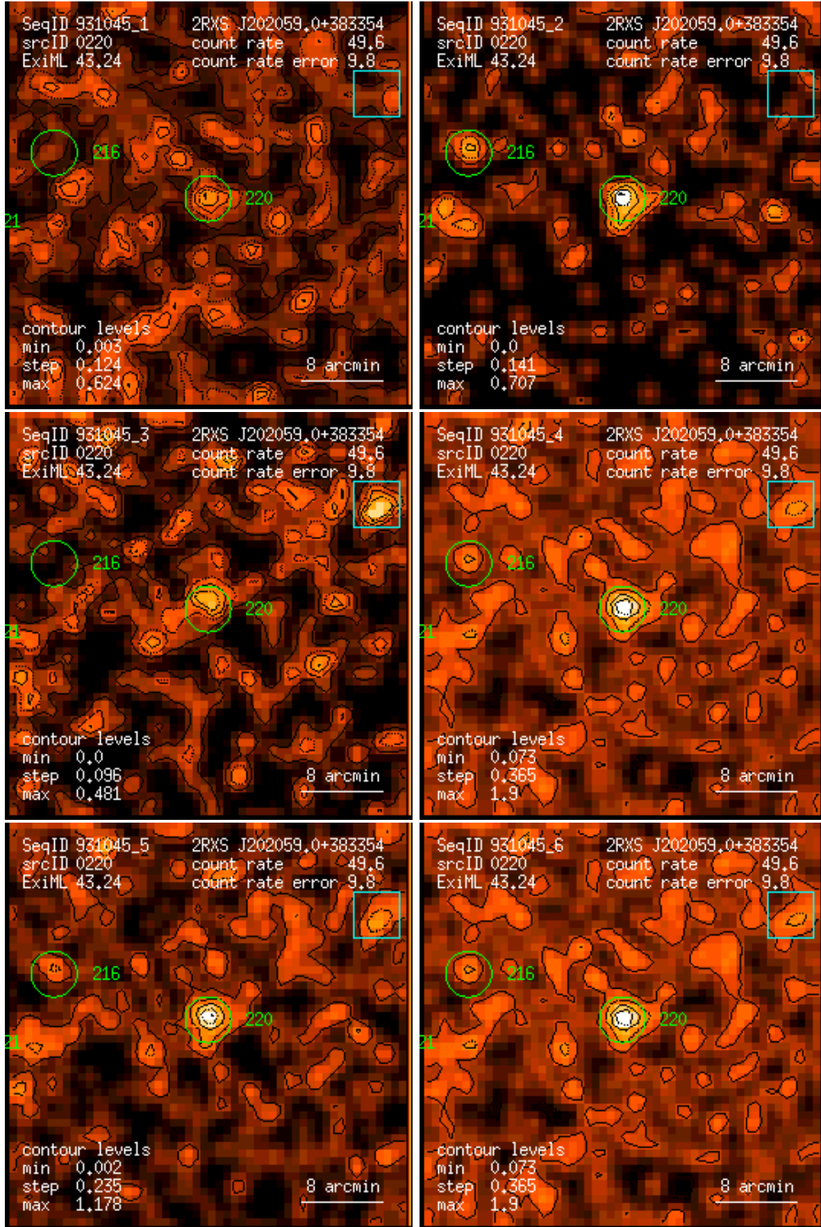
Figure 220: RASS 931045: detection 0220: band rate images, Gaussian filter: (1) PSPC channels 11 – 41, (2) 52 – 90, (3) 91 – 201, (4) 11 – 235, (5) 52 – 201, (6) 11 – 201. Broad band rates in counts/ks. Band rate contour levels in counts/ks/arcmin 2 .
