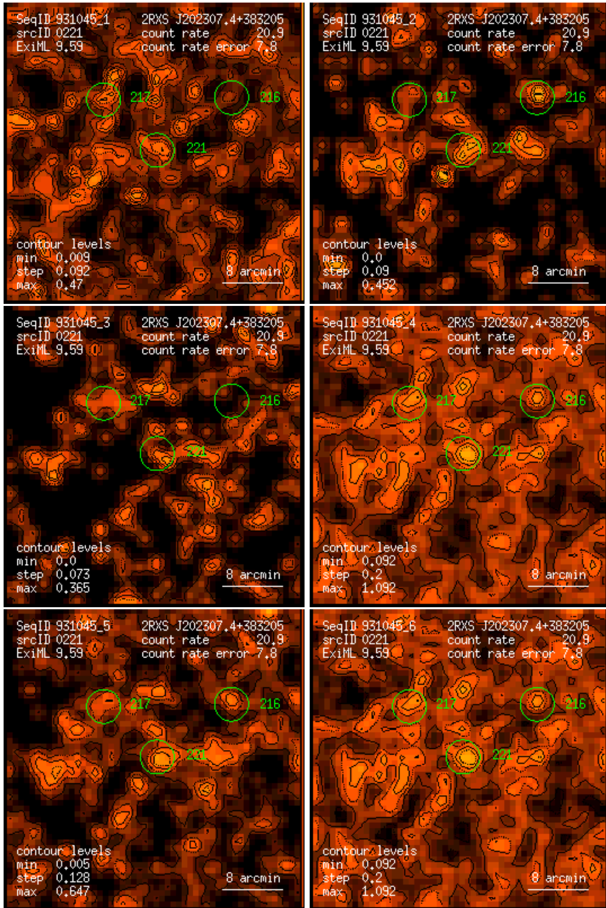
Figure 221: RASS 931045: detection 0221: band rate images, Gaussian filter: (1) PSPC channels 11 – 41, (2) 52 – 90, (3) 91 – 201, (4) 11 – 235, (5) 52 – 201, (6) 11 – 201. Broad band rates in counts/ks. Band rate contour levels in counts/ks/arcmin 2 .
