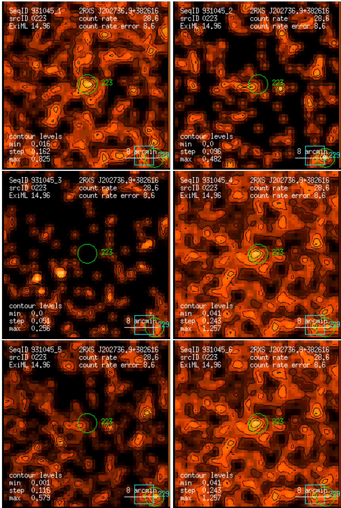
Figure 223: RASS 931045: detection 0223: band rate images, Gaussian filter: (1) PSPC channels 11 – 41, (2) 52 – 90, (3) 91 – 201, (4) 11 – 235, (5) 52 – 201, (6) 11 – 201. Broad band rates in counts/ks. Band rate contour levels in counts/ks/arcmin 2 .
