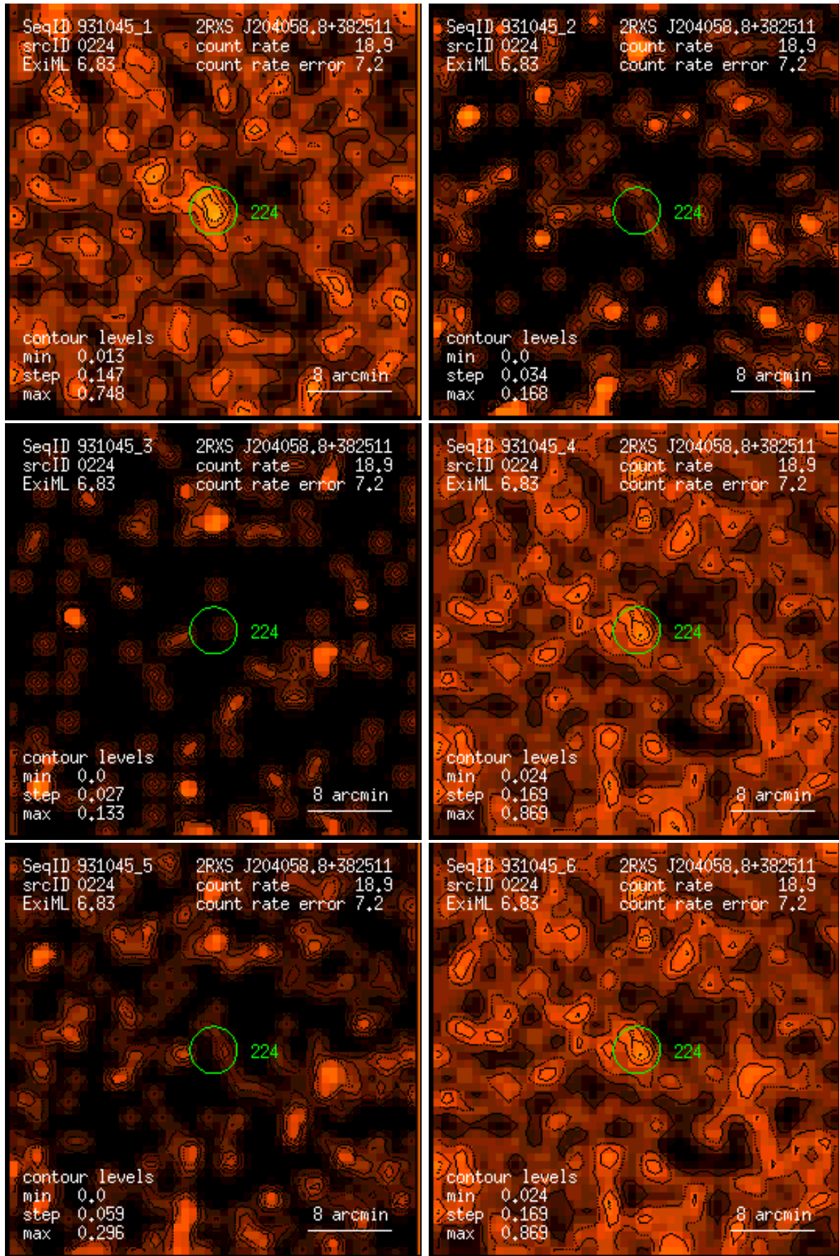
Figure 224: RASS 931045: detection 0224: band rate images, Gaussian filter: (1) PSPC channels 11 – 41, (2) 52 – 90, (3) 91 – 201, (4) 11 – 235, (5) 52 – 201, (6) 11 – 201. Broad band rates in counts/ks. Band rate contour levels in counts/ks/arcmin 2 .
