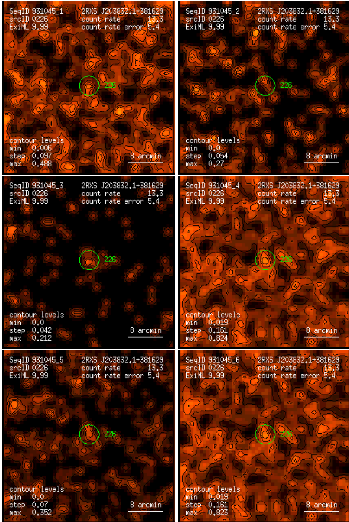
Figure 226: RASS 931045: detection 0226: band rate images, Gaussian filter: (1) PSPC channels 11 – 41, (2) 52 – 90, (3) 91 – 201, (4) 11 – 235, (5) 52 – 201, (6) 11 – 201. Broad band rates in counts/ks. Band rate contour levels in counts/ks/arcmin 2 .
