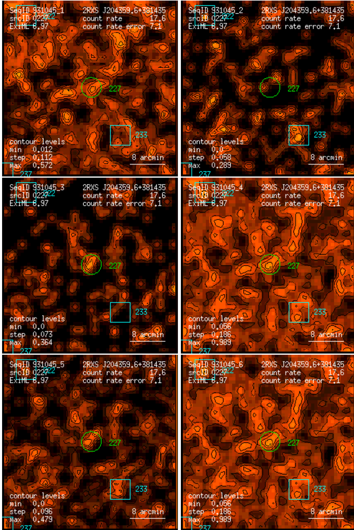
Figure 227: RASS 931045: detection 0227: band rate images, Gaussian filter: (1) PSPC channels 11 – 41, (2) 52 – 90, (3) 91 – 201, (4) 11 – 235, (5) 52 – 201, (6) 11 – 201. Broad band rates in counts/ks. Band rate contour levels in counts/ks/arcmin 2 .
