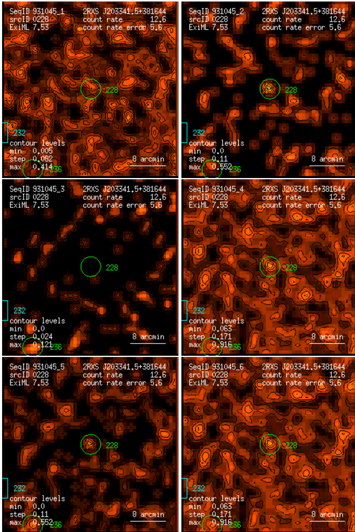
Figure 228: RASS 931045: detection 0228: band rate images, Gaussian filter: (1) PSPC channels 11 – 41, (2) 52 – 90, (3) 91 – 201, (4) 11 – 235, (5) 52 – 201, (6) 11 – 201. Broad band rates in counts/ks. Band rate contour levels in counts/ks/arcmin 2 .
