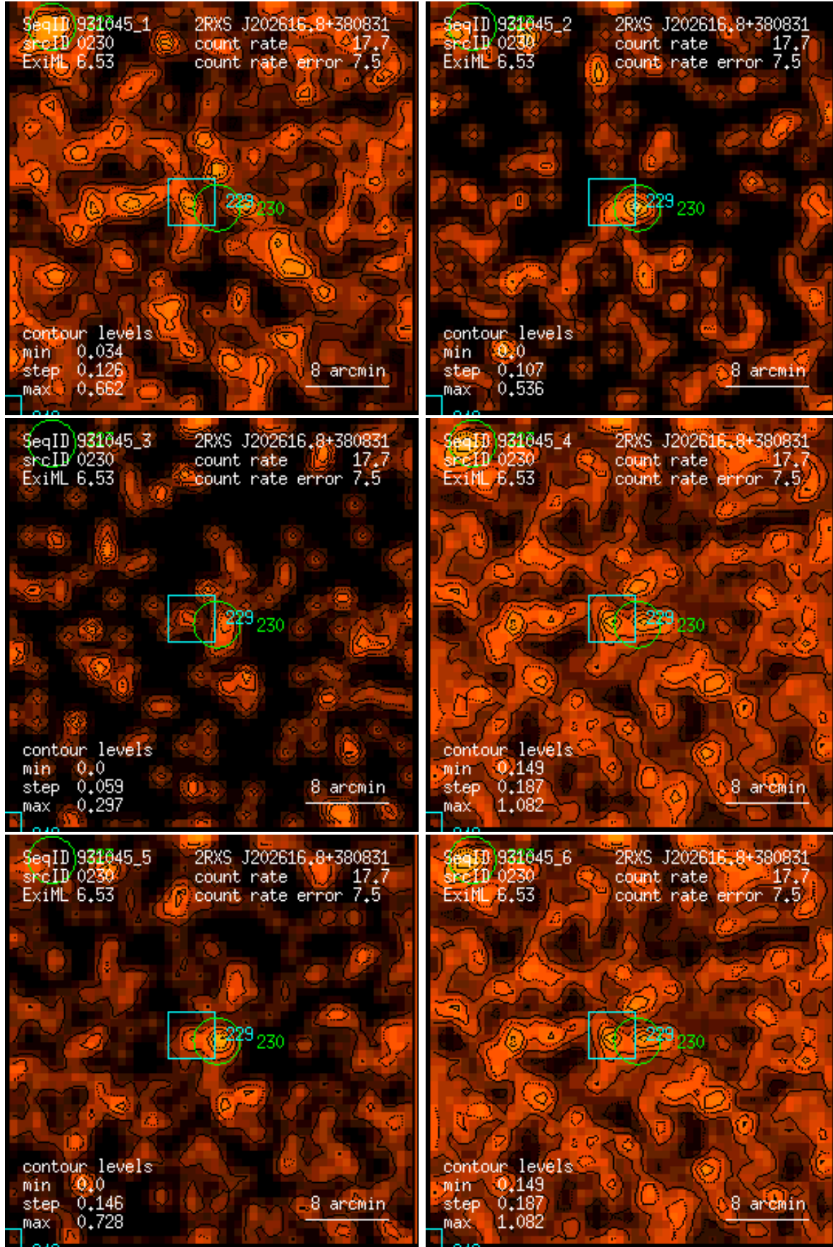
Figure 230: RASS 931045: detection 0230: band rate images, Gaussian filter: (1) PSPC channels 11 – 41, (2) 52 – 90, (3) 91 – 201, (4) 11 – 235, (5) 52 – 201, (6) 11 – 201. Broad band rates in counts/ks. Band rate contour levels in counts/ks/arcmin 2 .
