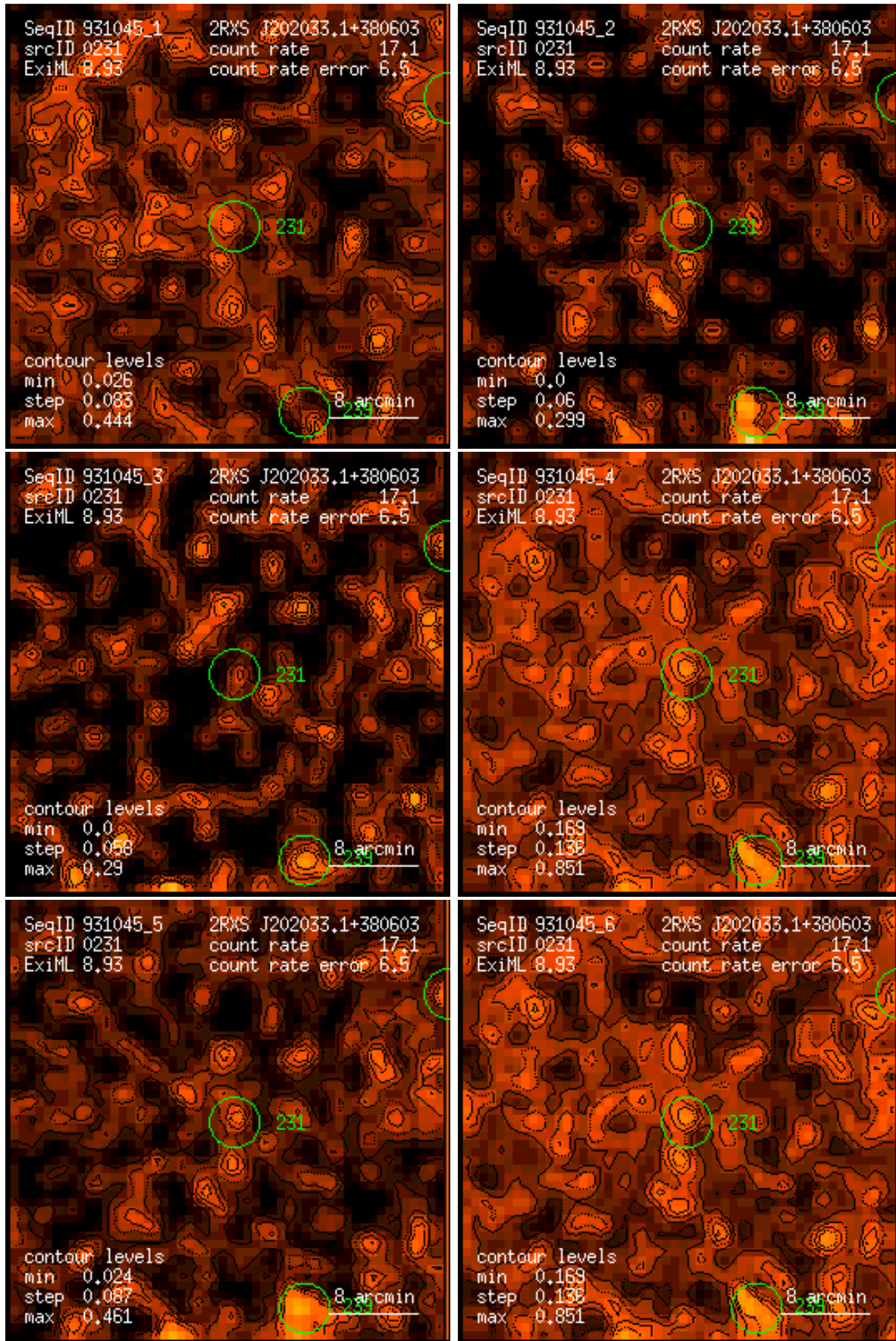
Figure 231: RASS 931045: detection 0231: band rate images, Gaussian filter: (1) PSPC channels 11 – 41, (2) 52 – 90, (3) 91 – 201, (4) 11 – 235, (5) 52 – 201, (6) 11 – 201. Broad band rates in counts/ks. Band rate contour levels in counts/ks/arcmin 2 .
