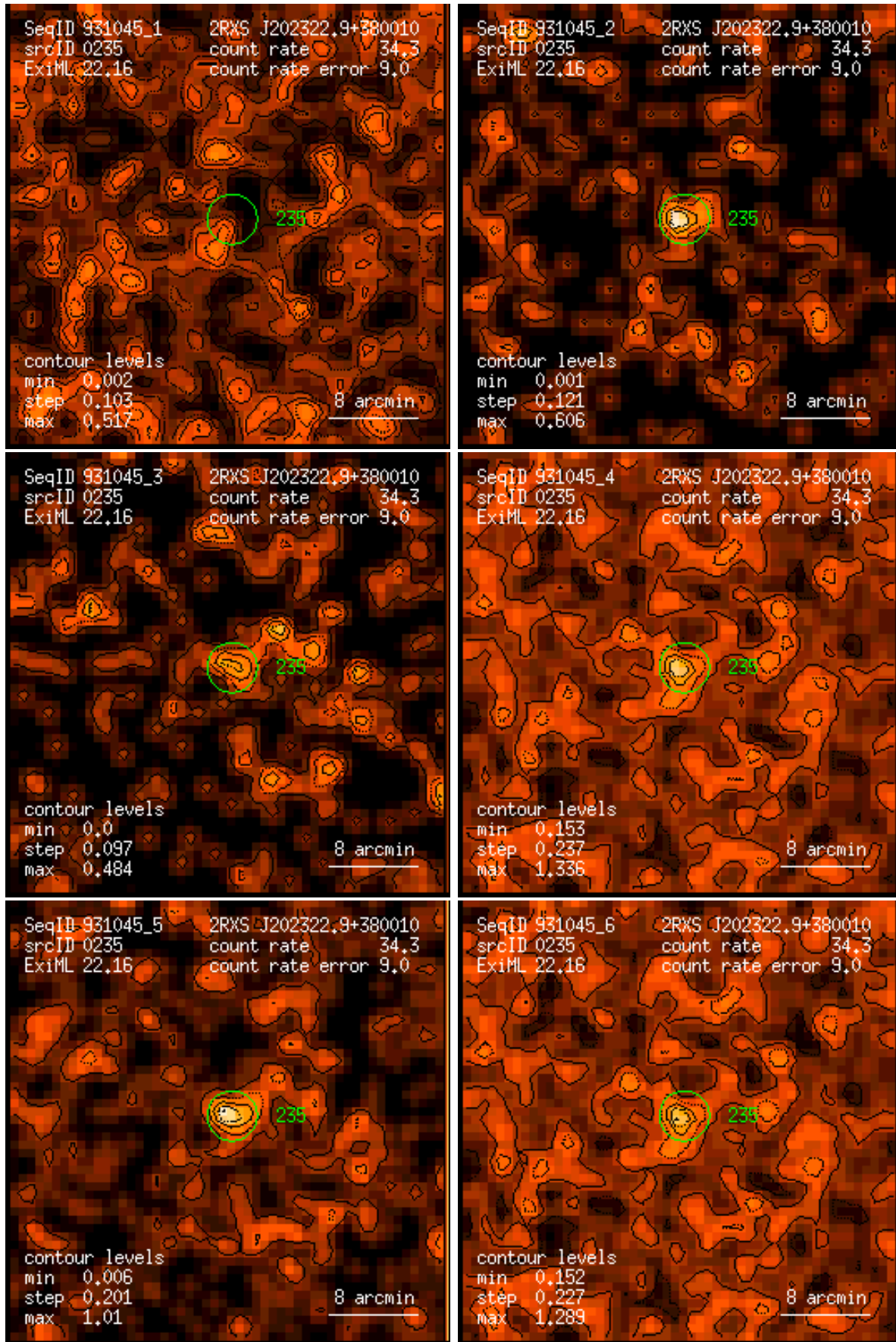
Figure 235: RASS 931045: detection 0235: band rate images, Gaussian filter: (1) PSPC channels 11 – 41, (2) 52 – 90, (3) 91 – 201, (4) 11 – 235, (5) 52 – 201, (6) 11 – 201. Broad band rates in counts/ks. Band rate contour levels in counts/ks/arcmin 2 .
