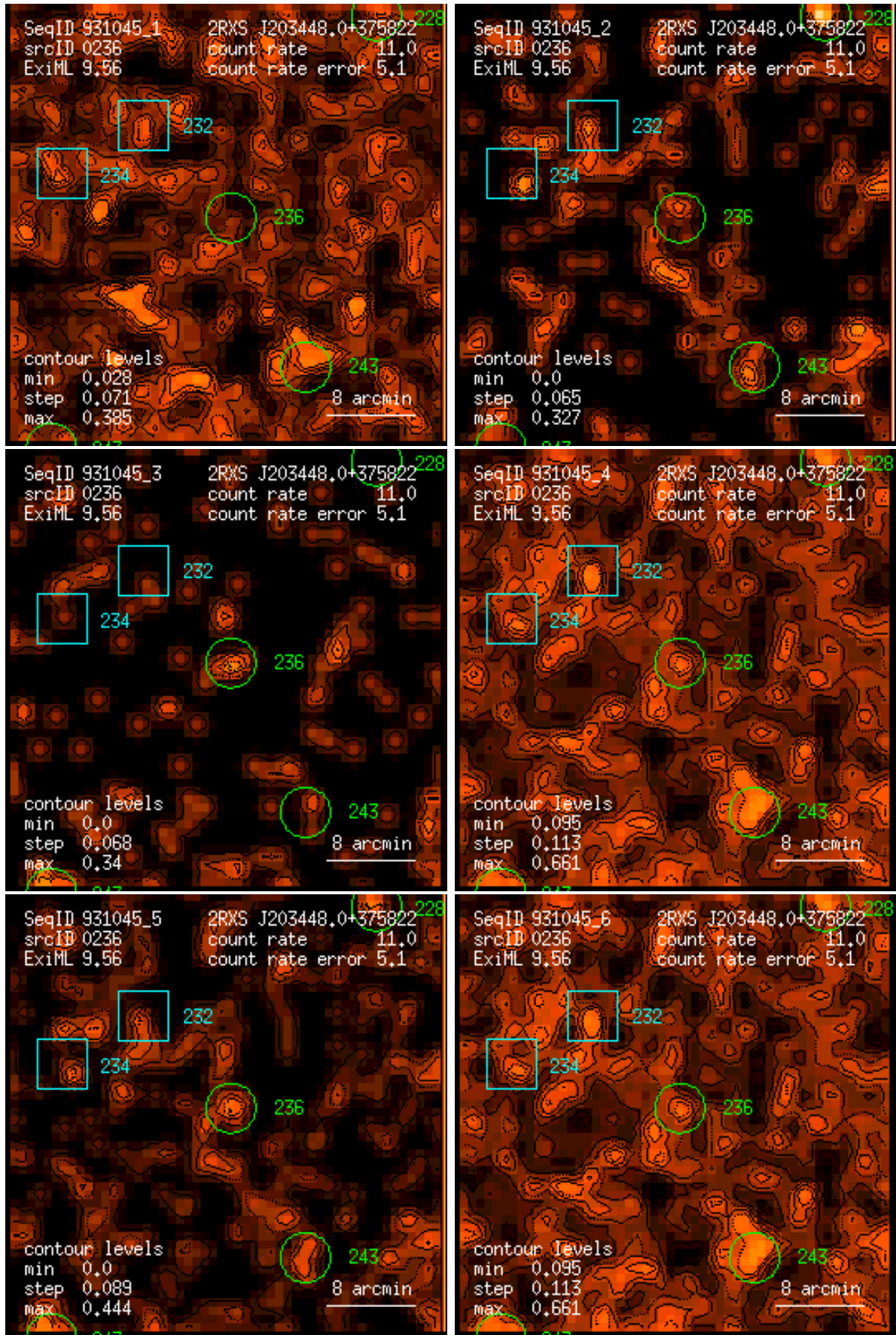
Figure 236: RASS 931045: detection 0236: band rate images, Gaussian filter: (1) PSPC channels 11 – 41, (2) 52 – 90, (3) 91 – 201, (4) 11 – 235, (5) 52 – 201, (6) 11 – 201. Broad band rates in counts/ks. Band rate contour levels in counts/ks/arcmin 2 .
