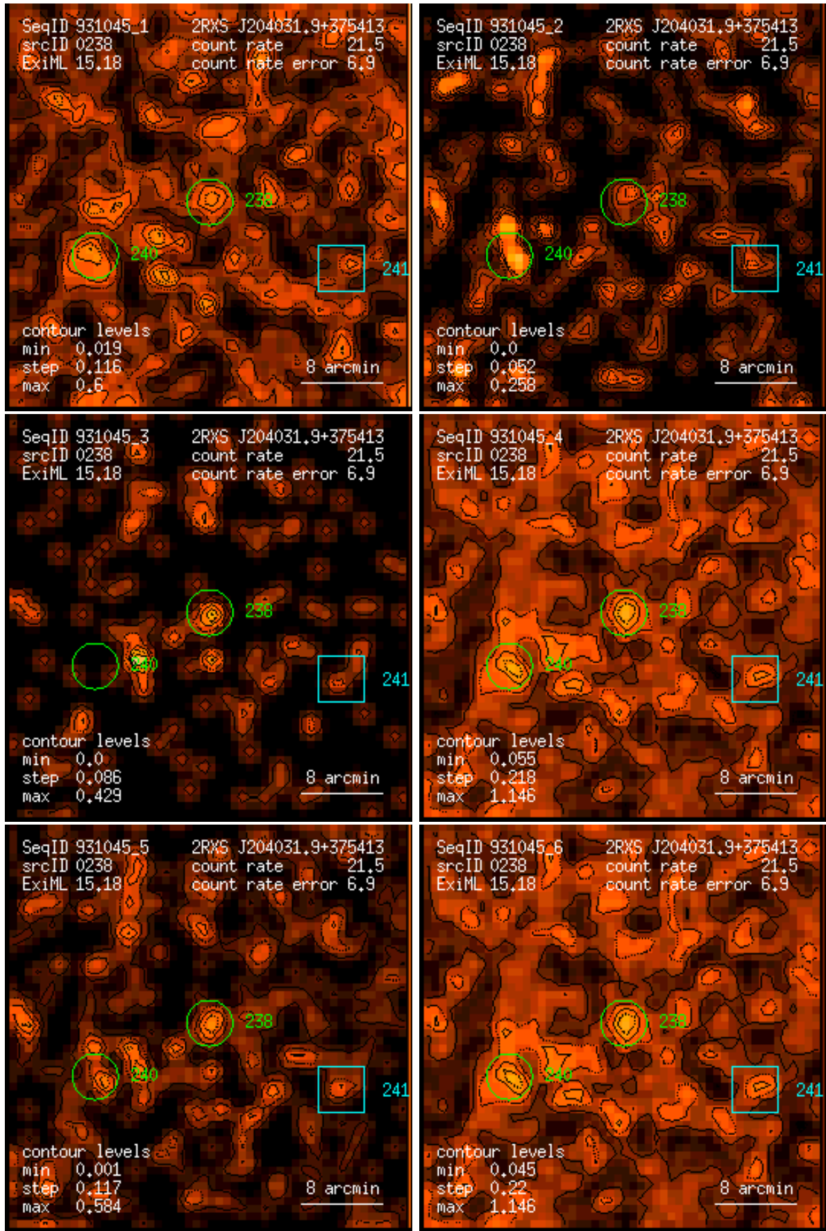
Figure 238: RASS 931045: detection 0238: band rate images, Gaussian filter: (1) PSPC channels 11 – 41, (2) 52 – 90, (3) 91 – 201, (4) 11 – 235, (5) 52 – 201, (6) 11 – 201. Broad band rates in counts/ks. Band rate contour levels in counts/ks/arcmin 2 .
