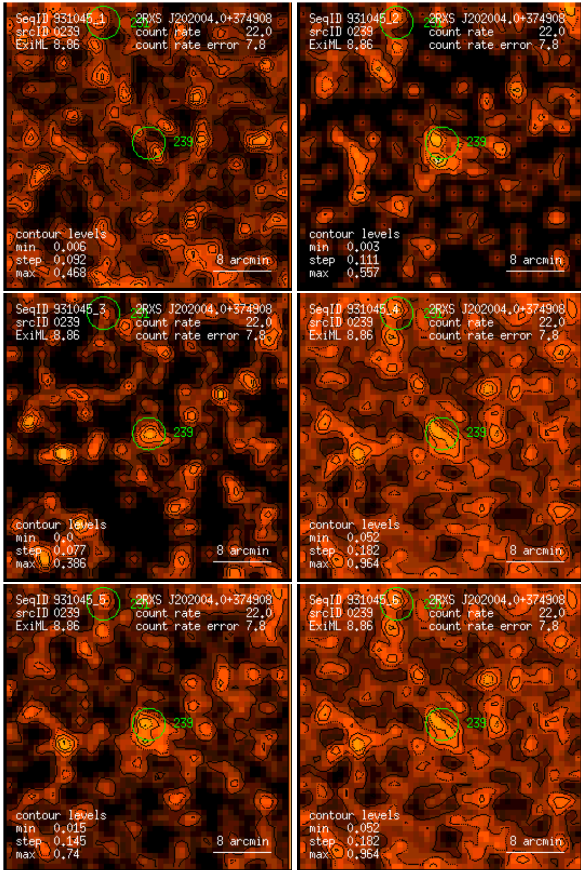
Figure 239: RASS 931045: detection 0239: band rate images, Gaussian filter: (1) PSPC channels 11 – 41, (2) 52 – 90, (3) 91 – 201, (4) 11 – 235, (5) 52 – 201, (6) 11 – 201. Broad band rates in counts/ks. Band rate contour levels in counts/ks/arcmin 2 .
