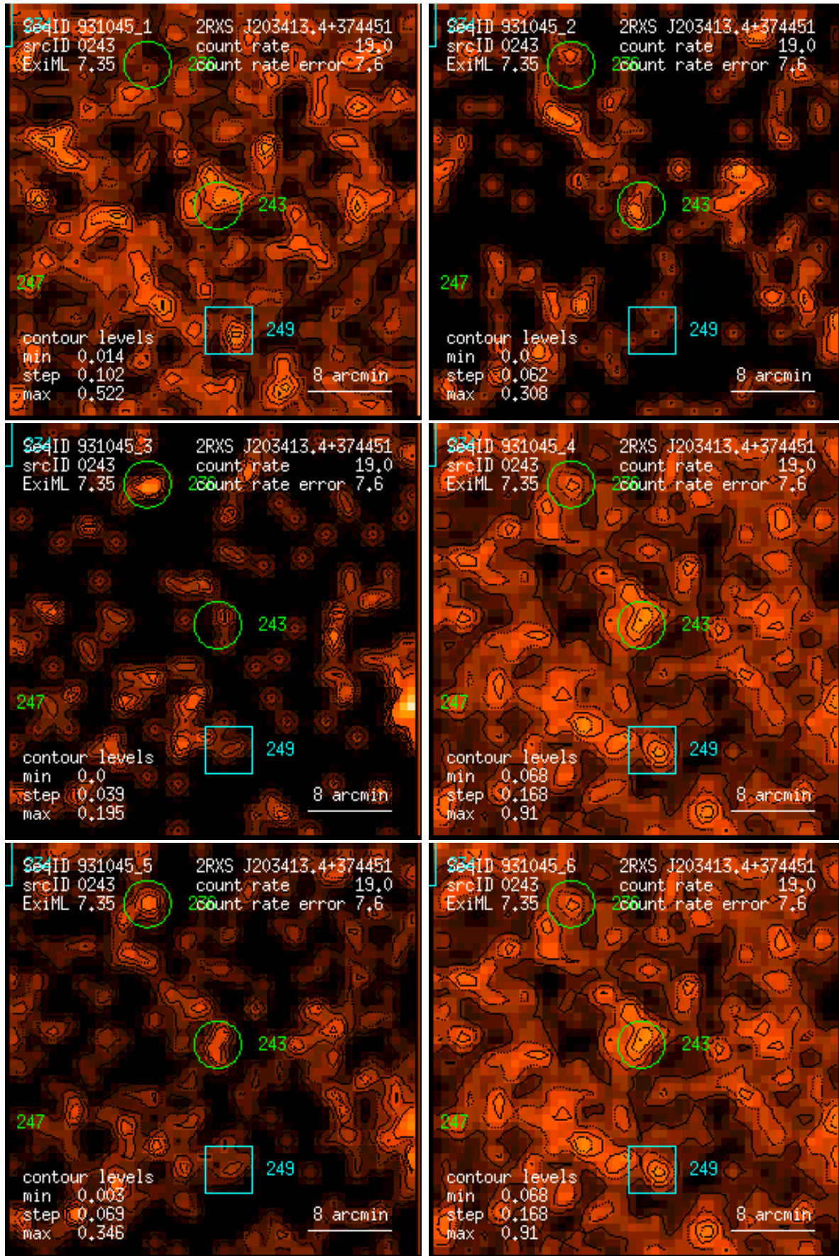
Figure 243: RASS 931045: detection 0243: band rate images, Gaussian filter: (1) PSPC channels 11 – 41, (2) 52 – 90, (3) 91 – 201, (4) 11 – 235, (5) 52 – 201, (6) 11 – 201. Broad band rates in counts/ks. Band rate contour levels in counts/ks/arcmin 2 .
