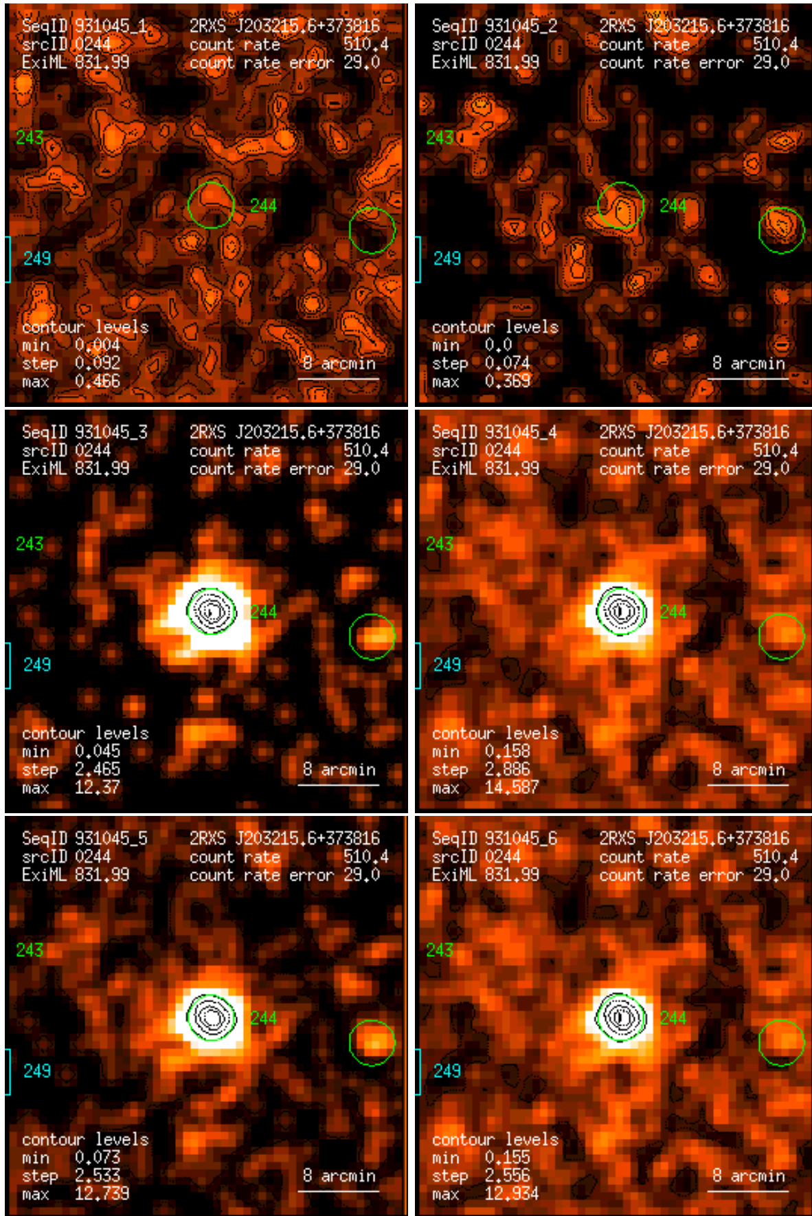
Figure 244: RASS 931045: detection 0244: band rate images, Gaussian filter: (1) PSPC channels 11 – 41, (2) 52 – 90, (3) 91 – 201, (4) 11 – 235, (5) 52 – 201, (6) 11 – 201. Broad band rates in counts/ks. Band rate contour levels in counts/ks/arcmin 2 .
