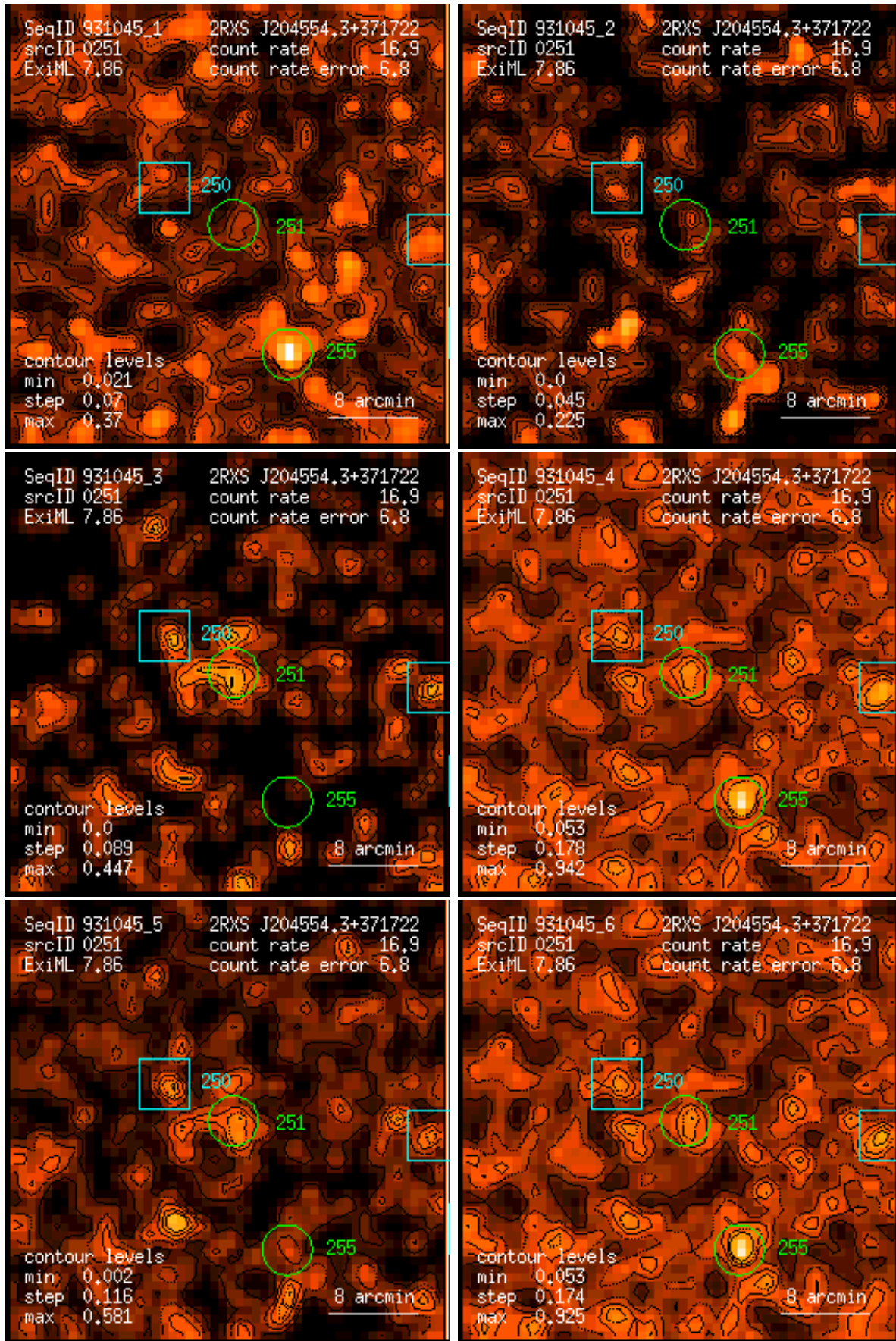
Figure 251: RASS 931045: detection 0251: band rate images, Gaussian filter: (1) PSPC channels 11 – 41, (2) 52 – 90, (3) 91 – 201, (4) 11 – 235, (5) 52 – 201, (6) 11 – 201. Broad band rates in counts/ks. Band rate contour levels in counts/ks/arcmin 2 .
