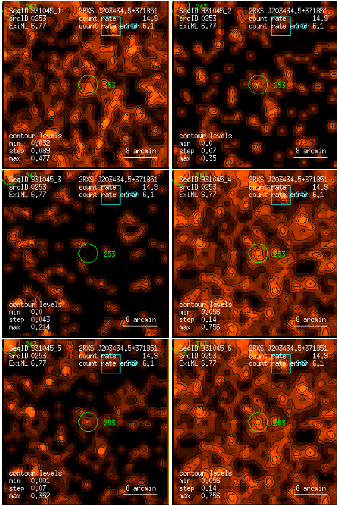
Figure 253: RASS 931045: detection 0253: band rate images, Gaussian filter: (1) PSPC channels 11 – 41, (2) 52 – 90, (3) 91 – 201, (4) 11 – 235, (5) 52 – 201, (6) 11 – 201. Broad band rates in counts/ks. Band rate contour levels in counts/ks/arcmin 2 .
