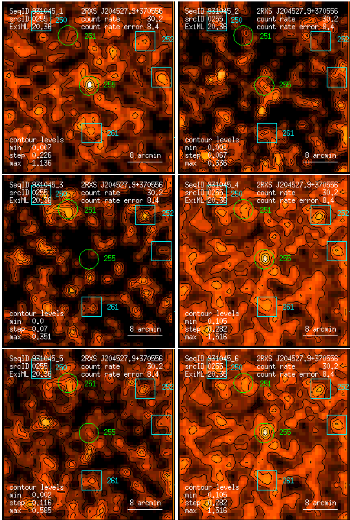
Figure 255: RASS 931045: detection 0255: band rate images, Gaussian filter: (1) PSPC channels 11 – 41, (2) 52 – 90, (3) 91 – 201, (4) 11 – 235, (5) 52 – 201, (6) 11 – 201. Broad band rates in counts/ks. Band rate contour levels in counts/ks/arcmin 2 .
