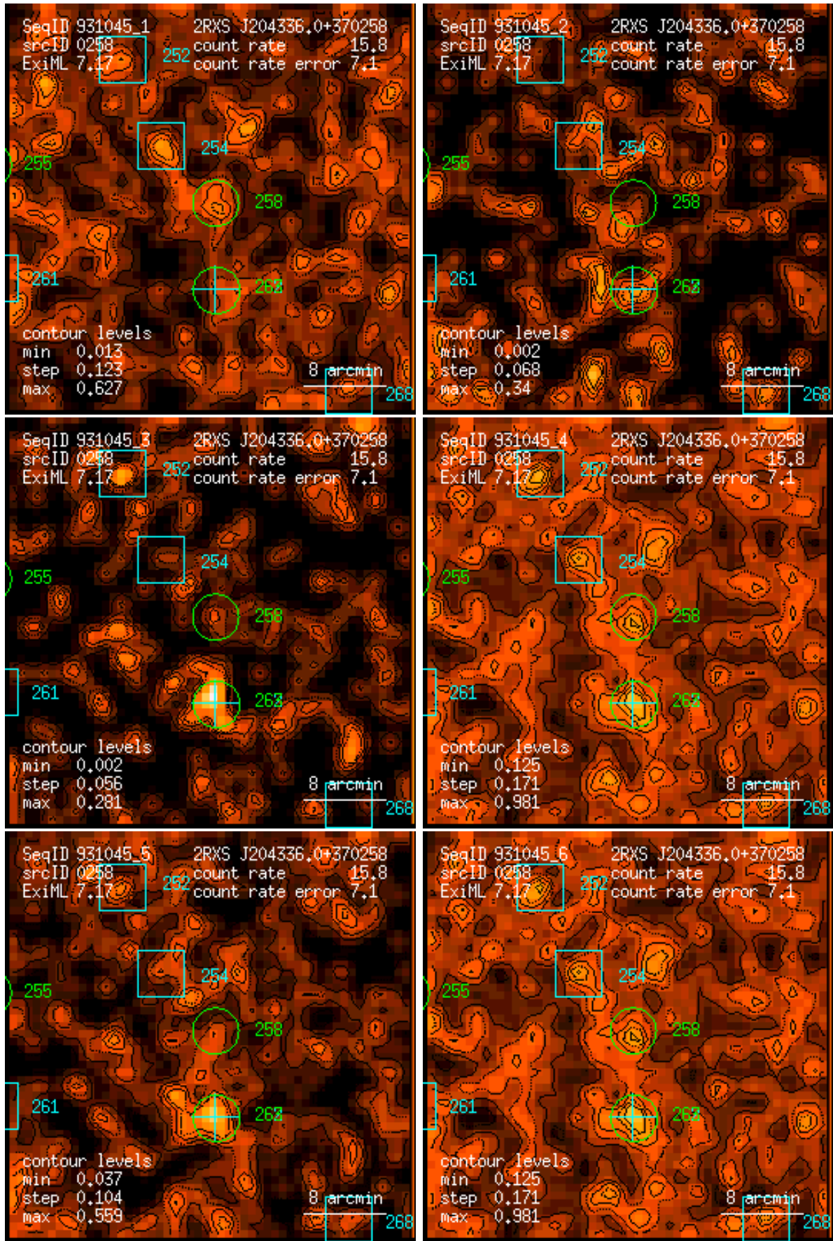
Figure 258: RASS 931045: detection 0258: band rate images, Gaussian filter: (1) PSPC channels 11 – 41, (2) 52 – 90, (3) 91 – 201, (4) 11 – 235, (5) 52 – 201, (6) 11 – 201. Broad band rates in counts/ks. Band rate contour levels in counts/ks/arcmin 2 .
