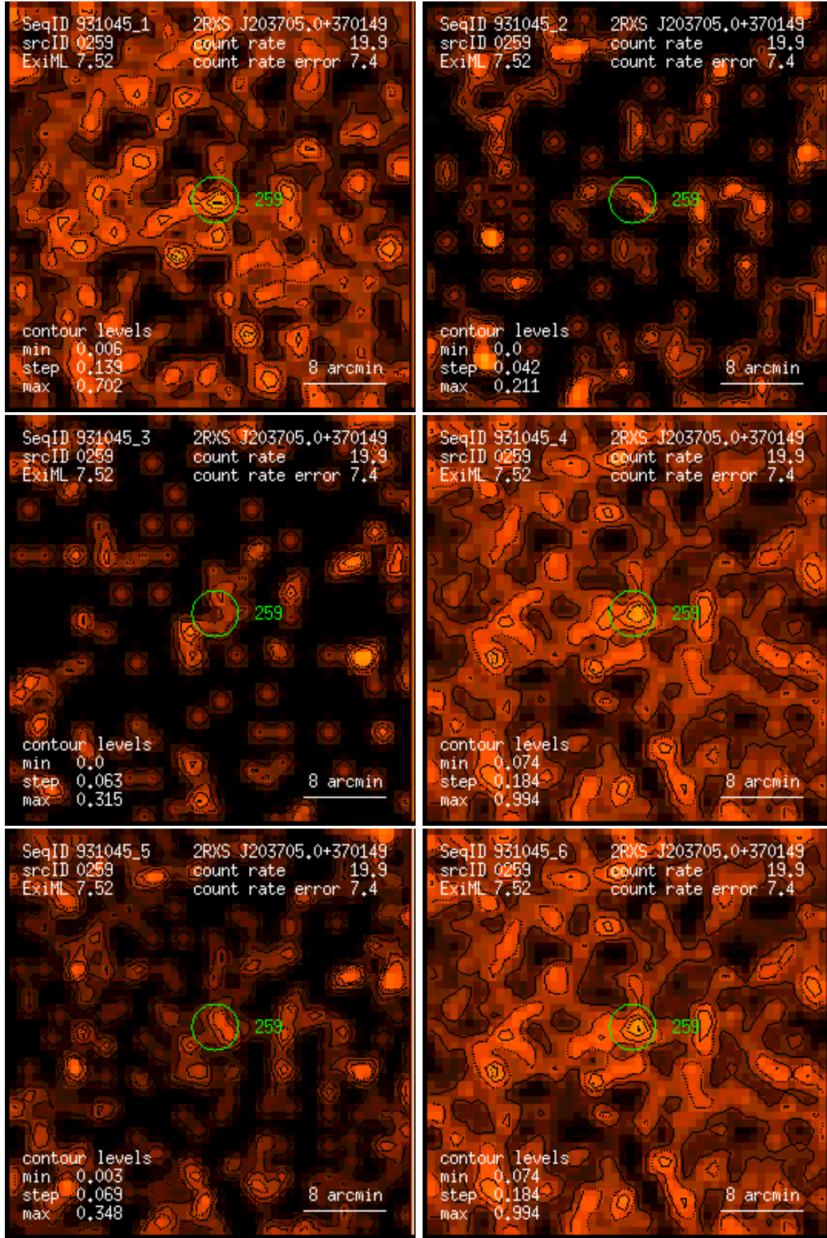
Figure 259: RASS 931045: detection 0259: band rate images, Gaussian filter: (1) PSPC channels 11 – 41, (2) 52 – 90, (3) 91 – 201, (4) 11 – 235, (5) 52 – 201, (6) 11 – 201. Broad band rates in counts/ks. Band rate contour levels in counts/ks/arcmin 2 .
