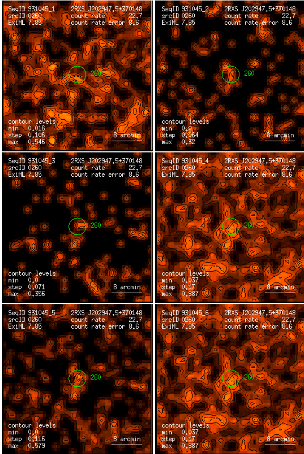
Figure 260: RASS 931045: detection 0260: band rate images, Gaussian filter: (1) PSPC channels 11 – 41, (2) 52 – 90, (3) 91 – 201, (4) 11 – 235, (5) 52 – 201, (6) 11 – 201. Broad band rates in counts/ks. Band rate contour levels in counts/ks/arcmin 2 .
