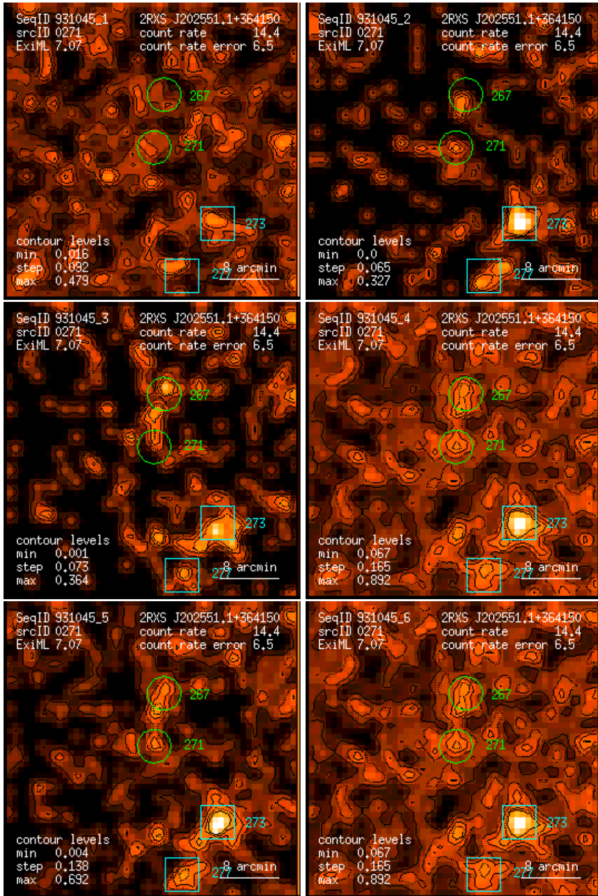
Figure 271: RASS 931045: detection 0271: band rate images, Gaussian filter: (1) PSPC channels 11 – 41, (2) 52 – 90, (3) 91 – 201, (4) 11 – 235, (5) 52 – 201, (6) 11 – 201. Broad band rates in counts/ks. Band rate contour levels in counts/ks/arcmin 2 .
