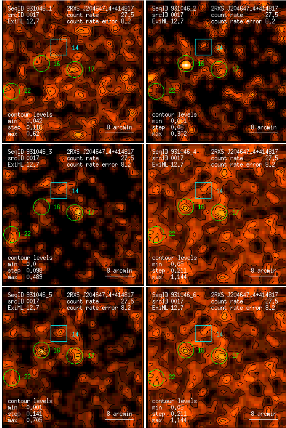
Figure 17: RASS 931046: detection 0017: band rate images, Gaussian filter: (1) PSPC channels 11 – 41, (2) 52 – 90, (3) 91 – 201, (4) 11 – 235, (5) 52 – 201, (6) 11 – 201. Broad band rates in counts/ks. Band rate contour levels in counts/ks/arcmin 2 .
