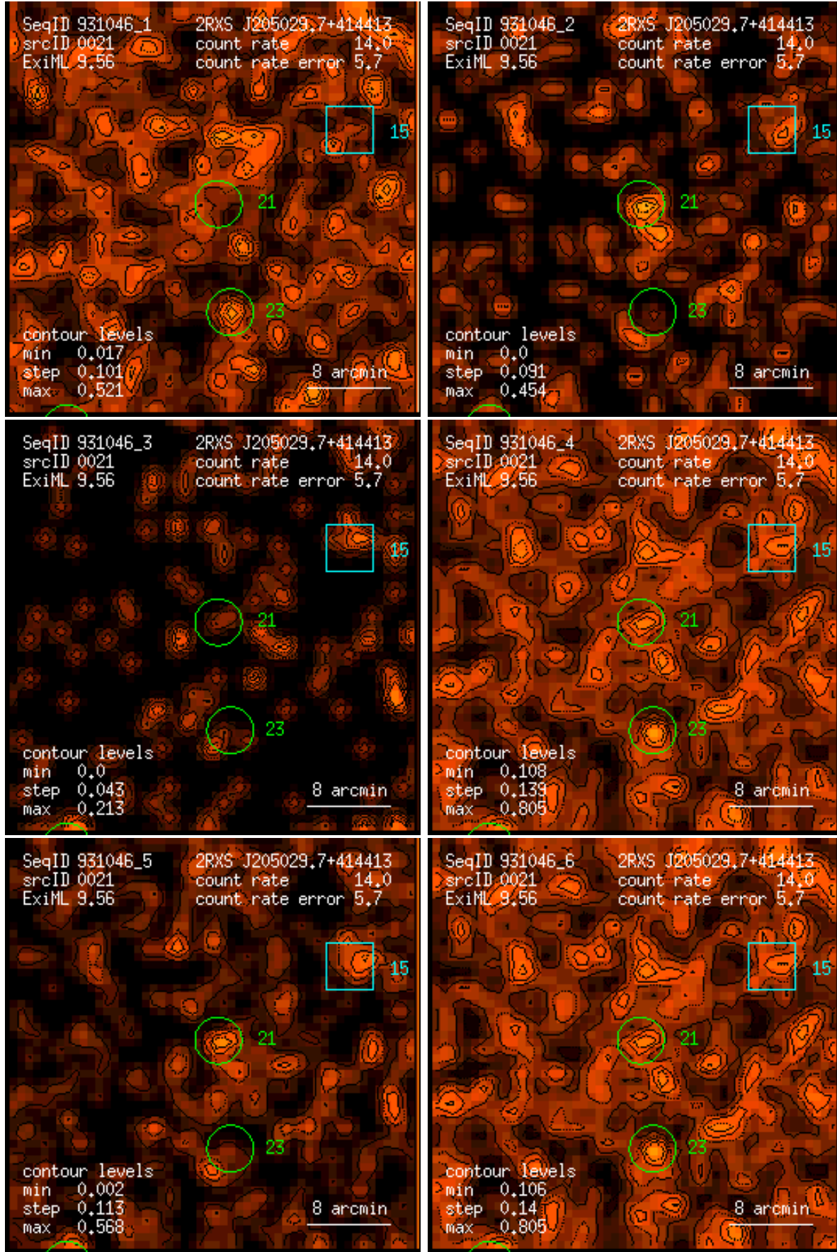
Figure 21: RASS 931046: detection 0021: band rate images, Gaussian filter: (1) PSPC channels 11 – 41, (2) 52 – 90, (3) 91 – 201, (4) 11 – 235, (5) 52 – 201, (6) 11 – 201. Broad band rates in counts/ks. Band rate contour levels in counts/ks/arcmin 2 .
